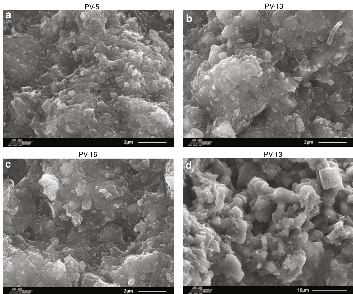
Figure 7. SEM images of halloysite (a–c) and gibbsite (d). Halloysites are from low terrace (a), upper terrace (b) and residual soil (c).
