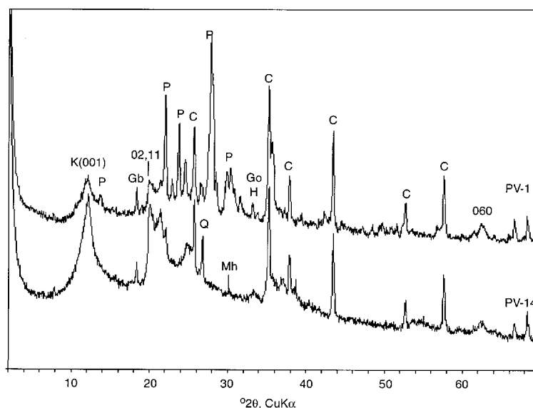
Figure 2. XRD analysis of bulk soils (B horizons) for samples PV-1 (upper pattern) and PV-14 (lower pattern). P = plagioclase, K(001) = 7 Å kaolin peak (halloysite + kaolinite), Q = quartz, C = corundum (internal std), Gb = gibbsite, Go = goethite, H = hematite, Mh = maghemite, 02,11 and 060 are kaolin reflections.
