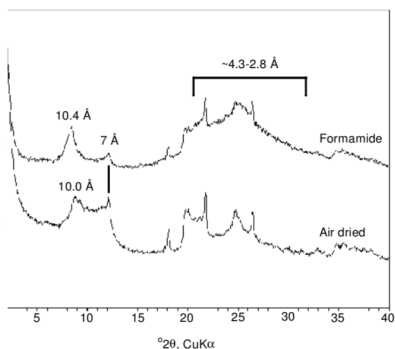
Figure 5. XRD analyses of oriented mounts of formamide-solvated powder (2–5 \mu\text{m} fraction, PV-14).
