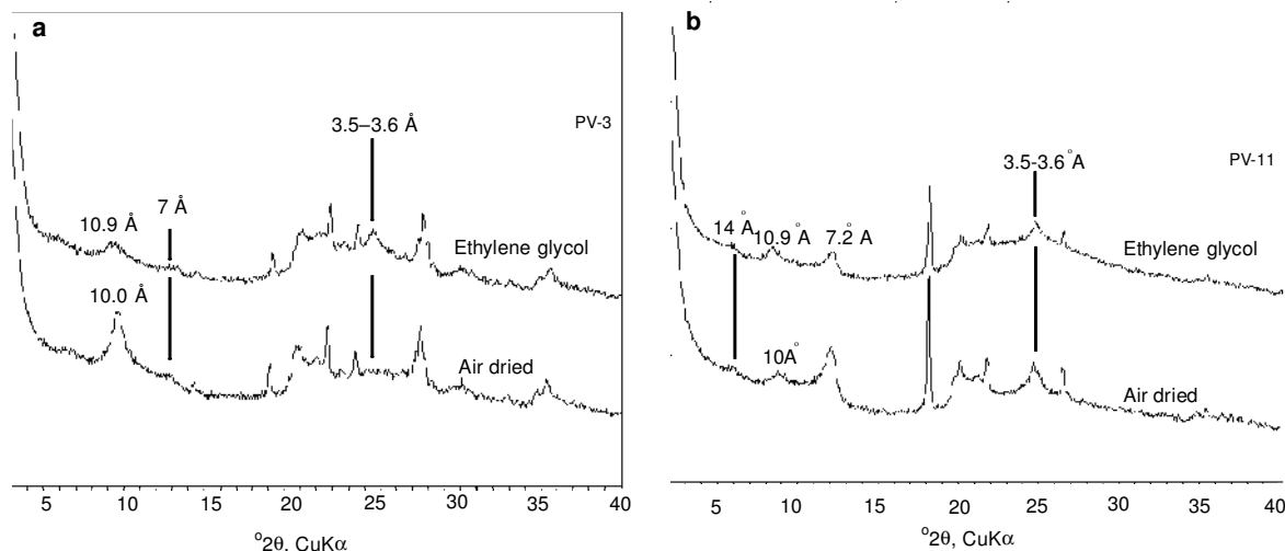
Figure 4. XRD analyses of oriented mounts of representative ethylene glycol-solvated powders (2–5 \mu\text{m} fraction). (a) = PV-3, (b) = PV-11.
