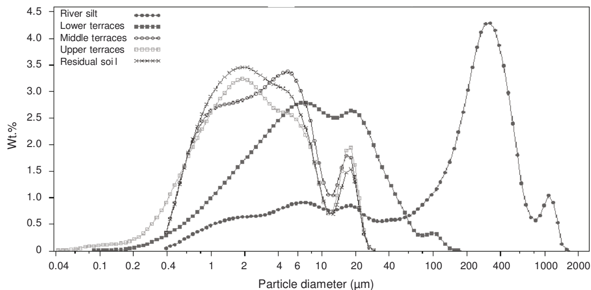
Figure 1. Variations in particle size of soil B horizons as a function of age, as determined by laser-diffraction particle-size analysis.
