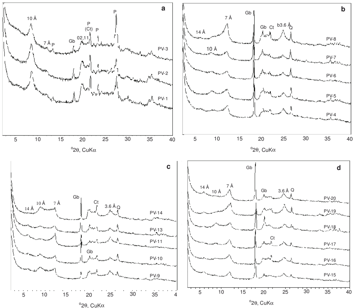
Figure 3. XRD analyses of oriented mounts of air-dried powders, 2–5 \mu\text{m} fraction. Sample numbers are indicated on the right and increase in age upwards. Approximate peak positions are given in \text{\AA} , P = plagioclase, Gb = gibbsite, 02,11 = kaolin reflections, Ct = cristobalite, Q = quartz. (a) Active floodplains, (b) low and middle terraces, (c) upper terraces, and (d) residual soils.
