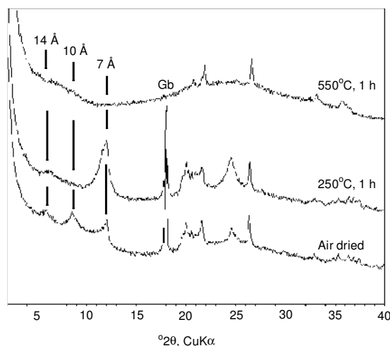
Figure 6. XRD analyses of oriented mounts heated to 250°C and 550°C for 1 h each (2–5 \mu\text{m} fraction, PV-10). Note the disappearance of gibbsite (Gb) and kaolin (7 Å) at 550°C.
