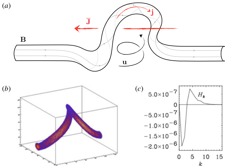
FIGURE 27. (a) Sketch of the dynamics of a magnetic flux tube in Parker's mechanism for a right-handed helical velocity fluctuation \mathbf{u} , showing a left-handed large-scale magnetic writhe associated with a large-scale current \mathbf{J} , and a right-handed internal twist associated with a small-scale current \mathbf{j} . This particular configuration is generally thought to be representative of the dynamics in the southern hemisphere of rotating stars with a strongly stratified convection zone, where motions have a net cyclonic bias (§4.4.1). (b,c) Computation of the Cauchy solution of an initially straight magnetic flux tube in a cyclonic velocity field (b), and corresponding magnetic-helicity spectrum (c) (adapted from Yousef & Brandenburg 2003).
