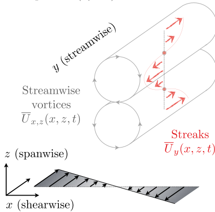
FIGURE 38. Comparison of the first stage of the hydrodynamic shear flow and instability-driven dynamo SSPs in the shearing sheet geometry. (a) Formation of streamwise-independent streaks of streamwise velocity \bar{U}_y(x, z, t) (red arrows) by the lift-up effect in the hydro SSP. The full red circles show the locations of two inflexion points of the streaky flow profile along z . (b) Amplification of azimuthal/toroidal magnetic field \bar{B}_y(x, z, t) by the \Omega effect in the dynamo SSP (red arrows).
