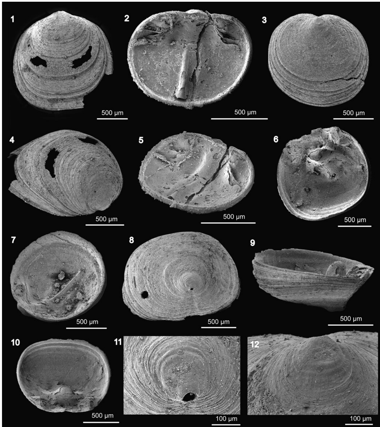
Figure 9. Batenevotreta? mexicana n. sp., from the El Gavilán Formation (sample SJG 2/9), Cambrian (Wuliuan), Chihuarruita Hill outcrop, Mexico. (1, 4) (USTL4040-1) (1) Dorsal valve exterior, (4) oblique posterolateral view; (2, 5) (USTL4040-2) (2) dorsal valve interior; (3) (USTL4040-3) ventral valve exterior, (5), oblique anterolateral view; (6, 9, 10) (USTL4040-4) ventral valve interior, (9) oblique lateral view, (10) oblique posterior view; (7) (USTL4040-5) oblique lateral view of dorsal valve interior; (8, 11, 12) (USTL4040-6) holotype, oblique posterolateral view of ventral valve exterior, (11) oblique posterolateral view of ventral metamorphic shell, (12) detail of umbo.
