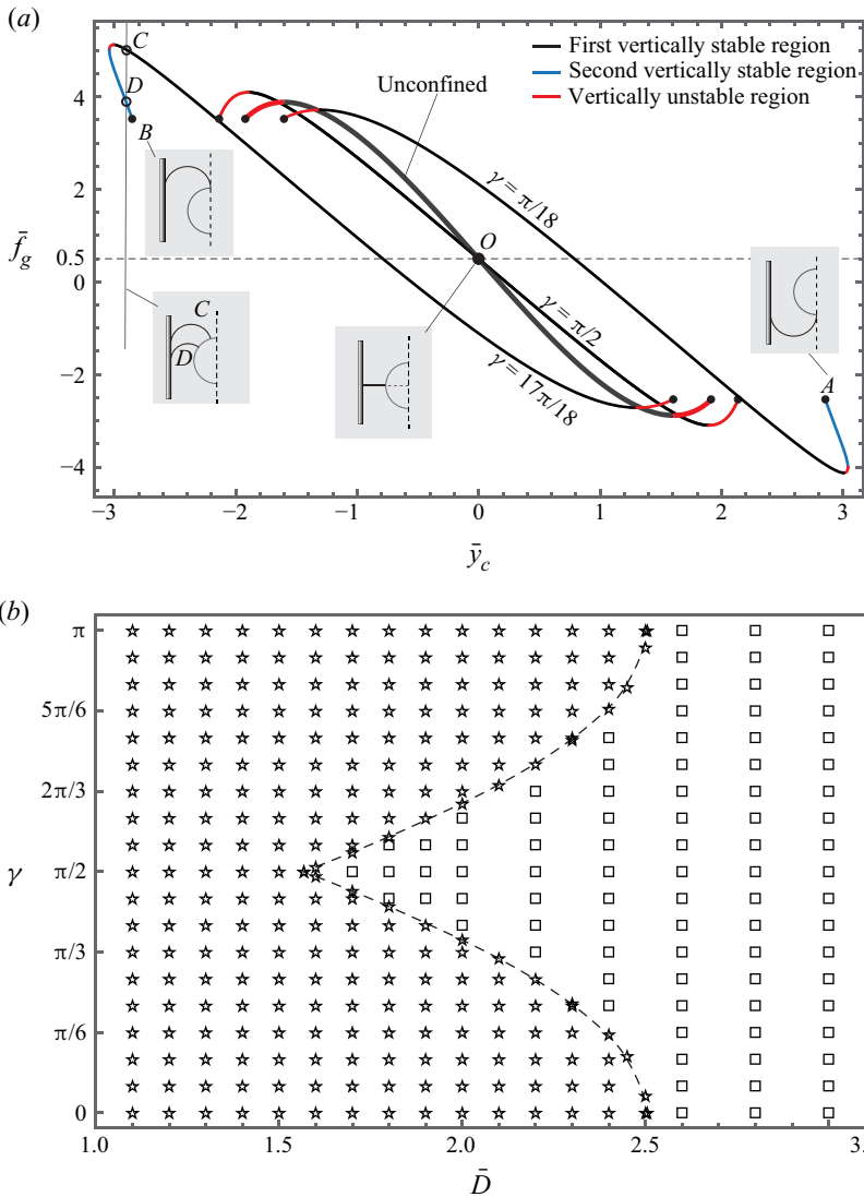
Figure 8. (a) Relation of \bar{f}_g and \bar{y}_c at the equilibria of fully symmetric menisci. The black curves and the blue curves denote vertically stable equilibria, while the red curves denote vertically unstable equilibria. The point A denotes the state of \alpha = -\pi/2 , the point B denotes the state of \alpha = \pi/2 and the point O denotes the states of the half-immersed cylinder with flat menisci. The two solution curves with plates' contact angles supplementary to each other (such as \gamma = \pi/18 and \gamma = 17\pi/18 ) are symmetric about the point O where (\bar{x}_c, \bar{y}_c, \bar{f}_g) = (\bar{D}/2, 0, 0.5) . The following parameters are used: \bar{D} = 2 , \bar{r} = 0.5 and \theta = \pi/2 . (b) Phase diagram of the equilibrium solutions of fully symmetric menisci with the first and the second vertical stability regions (denoted by pentagrams) and with only the first vertical stability region (denoted by squares), in a parameter space (\gamma, \bar{D}) for \bar{r} = 0.5 and \theta = \pi/2 . The occurrence of the second stability region for different \gamma in (a) can be checked by letting \bar{D} = 2 in (b).
