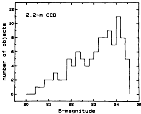
Fig. 2. Apparent luminosity function (in bins of 0.2 mag) for starlike objects around NGC 3115, from the 2.2-m CCD frames (central region of 2' \times 3' ).
