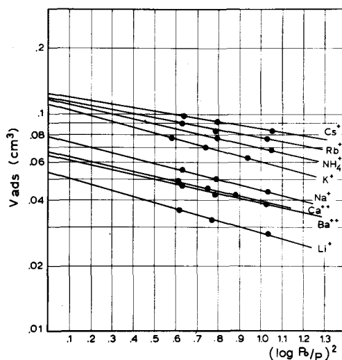
Fig. 3. Dubinin plots (see text).
