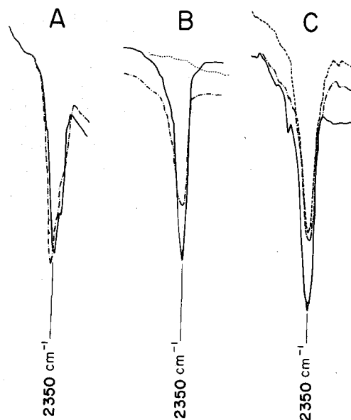
Fig. 2. I.R. transmission spectra of A: Li-smectite; B: K-smectite and C: Cs-smectite. Low temperature and normal incidence (—); low temperature and tilted by 35^{\circ} (---), room temperature and normal incidence (.....). Background in absence of CO 2 (— · — · —).
