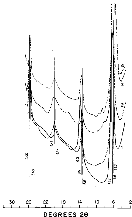
Fig. 1(b). Adsorption of CO 2 by Ca-smectite. X-ray (CuK \alpha ) diagrams obtained at different stages. (1) Outgassed for 2 hr at room temperature; (2) cooled in presence of 700 torr CO 2 at -20^{\circ}\text{C} ; (3) as (2), but at -63^{\circ}\text{C} ; (4) as (3), but rewarmed in presence of CO 2 at room temperature. Spacings for the main reflections are indicated.
