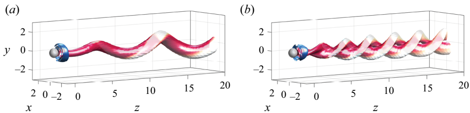
Figure 11. Three-dimensional structures of RW_1 (a) and RW_3 (b) at Re = 110 and \Omega = 1.75 . We have used isosurfaces of Q-criterion, Q = 0.001 , coloured by streamwise vorticity, \varpi_z \in [-1, 1] (blue to red) to depict the flow structure.
