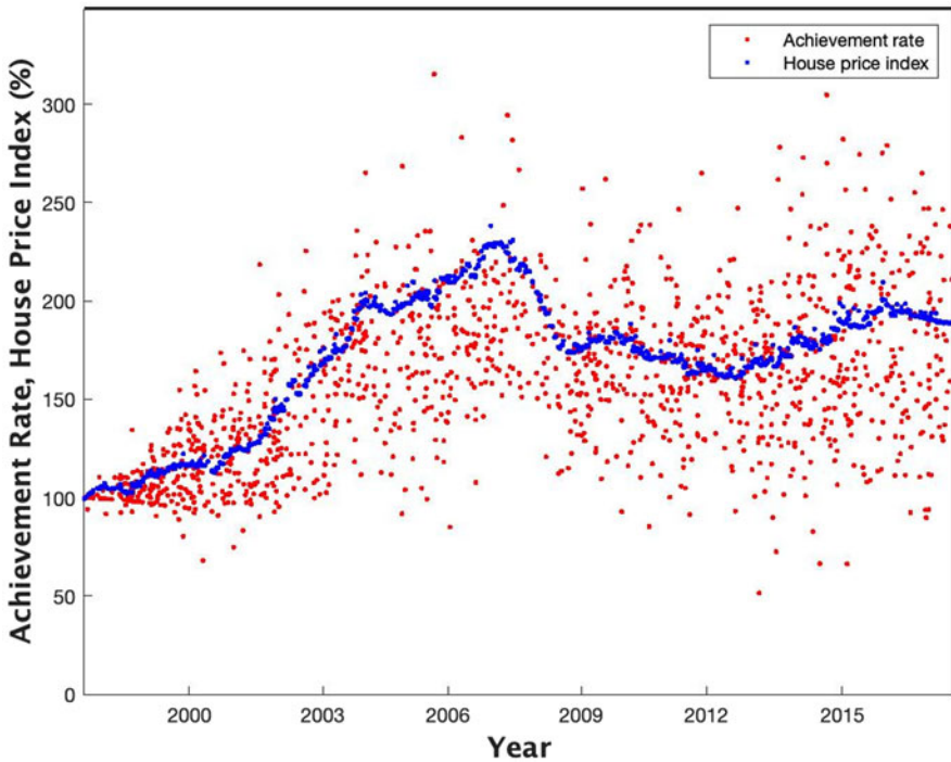
Figure 2. Indexed vs. achieved house prices. Source: SAMS.
