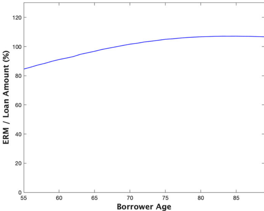
Figure 6. ERM /loan ratios vs. borrower age.
