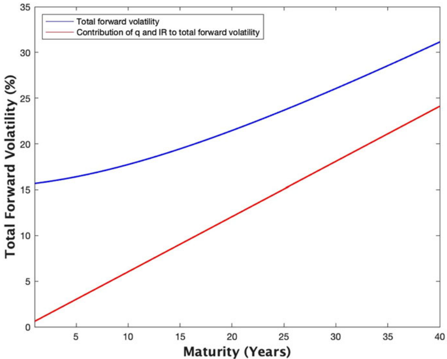
Figure 4. Term structure of total forward volatility.
