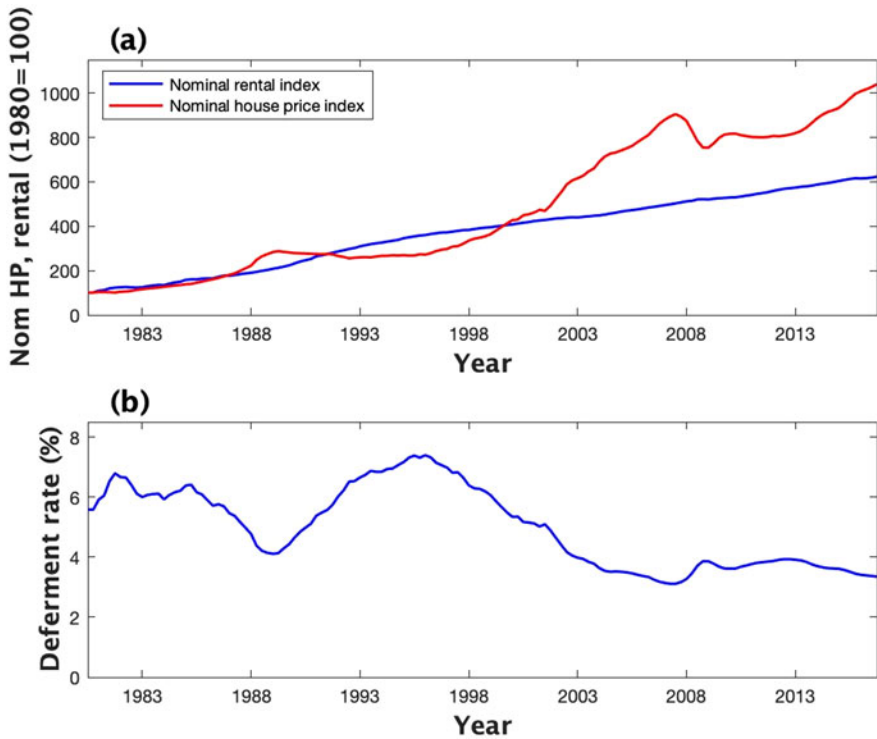
Figure 3. UK nominal house and rental indices and implied deferment rate. (a) UK nominal house prices and nominal rentals (b) Implied UK deferment rate. Source: OECD.
