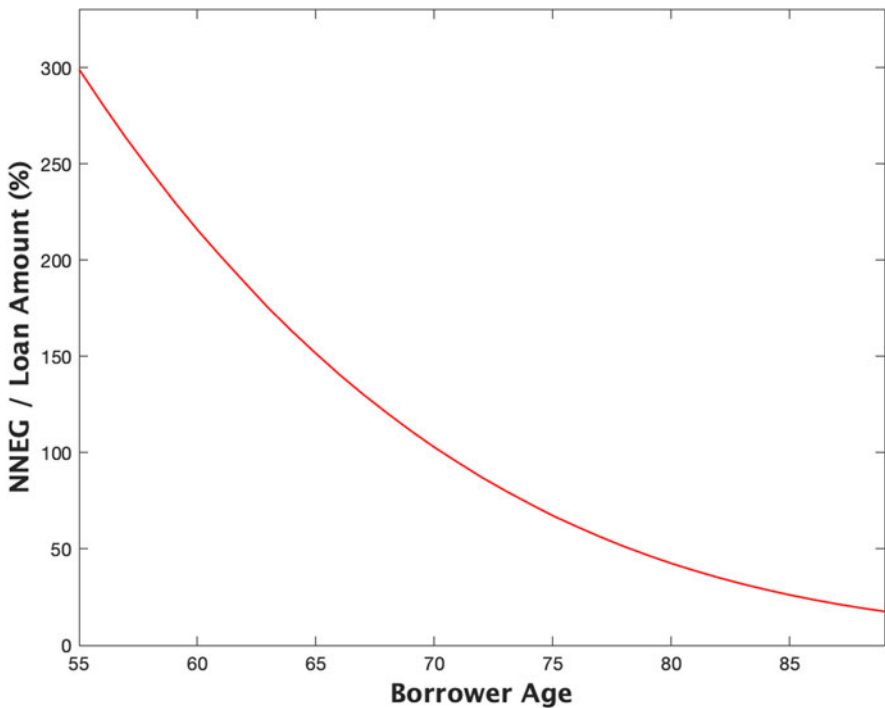
Figure 5. NNEG/loan ratios vs. borrower age.
