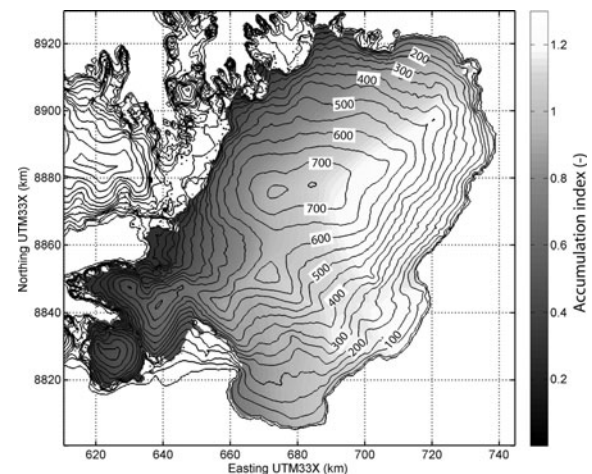
Fig. 3. The accumulation-index map used to distribute snow precipitation across Austfonna. Values are dimensionless and relative to the mean accumulation across the entire ice cap. See Taurisano and others (2007) for details. Contour lines show elevation (m a.s.l.); interval is 50 m.
