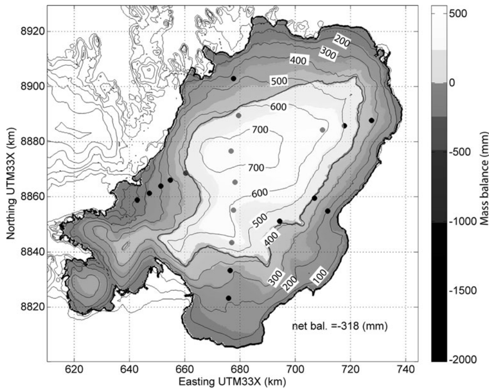
Fig. 6. The modelled distribution of surface mass balance for the period 29 April 2004 to 23 April 2005. The overall net balance is -318 mm. Accumulation is shown in light grey, and ablation is represented in dark grey. Dots indicate the locations of mass-balance stakes. Contour lines show elevation (m.a.s.l.); interval is 100 m.
