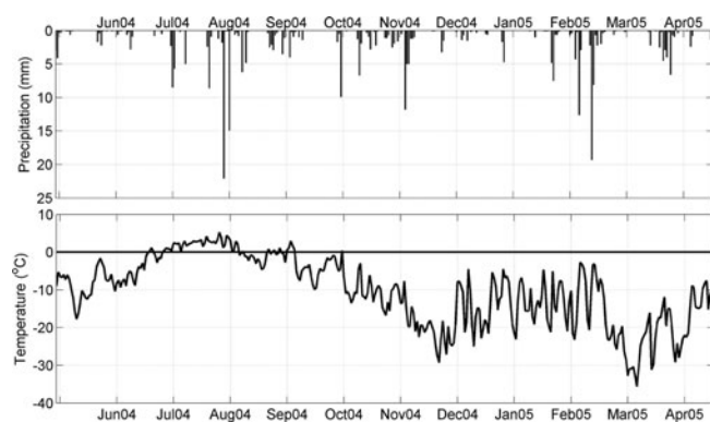
Fig. 2. Meteorological input data used to drive the mass-balance model. The top panel shows the diurnal precipitation at Ny-Ålesund, and the bottom panel shows daily mean temperatures recorded at 540 m a.s.l. on Austfonna.
