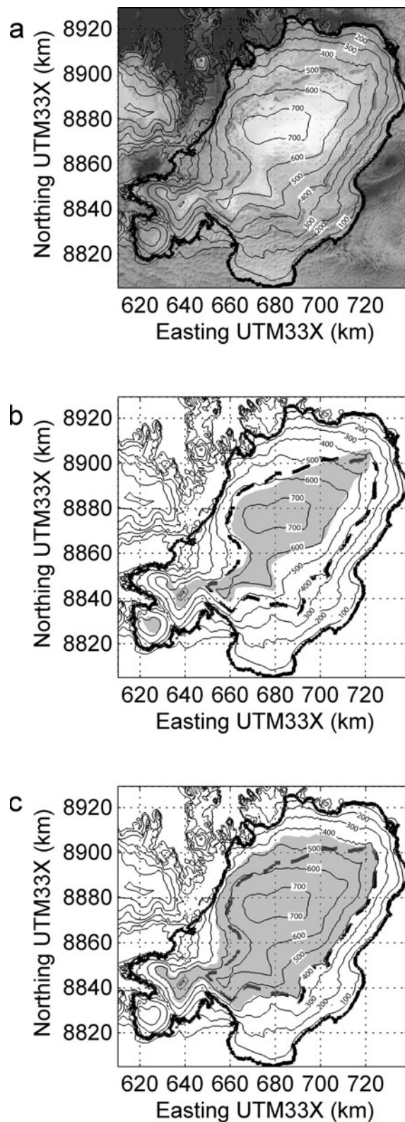
Fig. 4. Visual comparison of a MODIS image of 10 August 2004 (a) and the modelled extent of snow and firn for 10 August 2004 (snow and firn in grey): (b) best fit, and (c) due to incorrect snowmelt parameterization. See text for details. The stippled lines delineate the modelled accumulation area. The difference between the accumulation area and the snow/firn area visible in (a) and (b) is due to extensive formation of superimposed ice, especially in the southeast part of the ice cap. Contour lines show elevation (m.a.s.l.), interval is 100 m.
