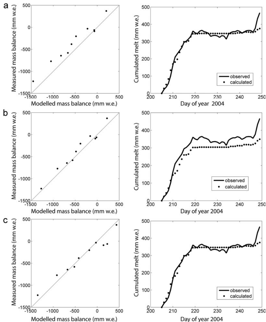
Fig. 5. Evaluating the model performance using scatter plots of modelled vs measured net mass balance at the stake locations (left column) and comparison of calculated and observed time series of melt (right column). Situations (a) and (b) were calculated neglecting refreezing ( P_{MAX} = 0 ). (a) shows a good estimate of the melt rate, but the modelled net balance is too negative. In contrast, the parameters used to calculate (b) yield a good correlation between modelled and measured net balance but underestimate the melt rate. (c) displays the model performance using the optimized parameter set, and refreezing is taken into account. Day 200 in 2004 corresponds to 18 July 2004.
