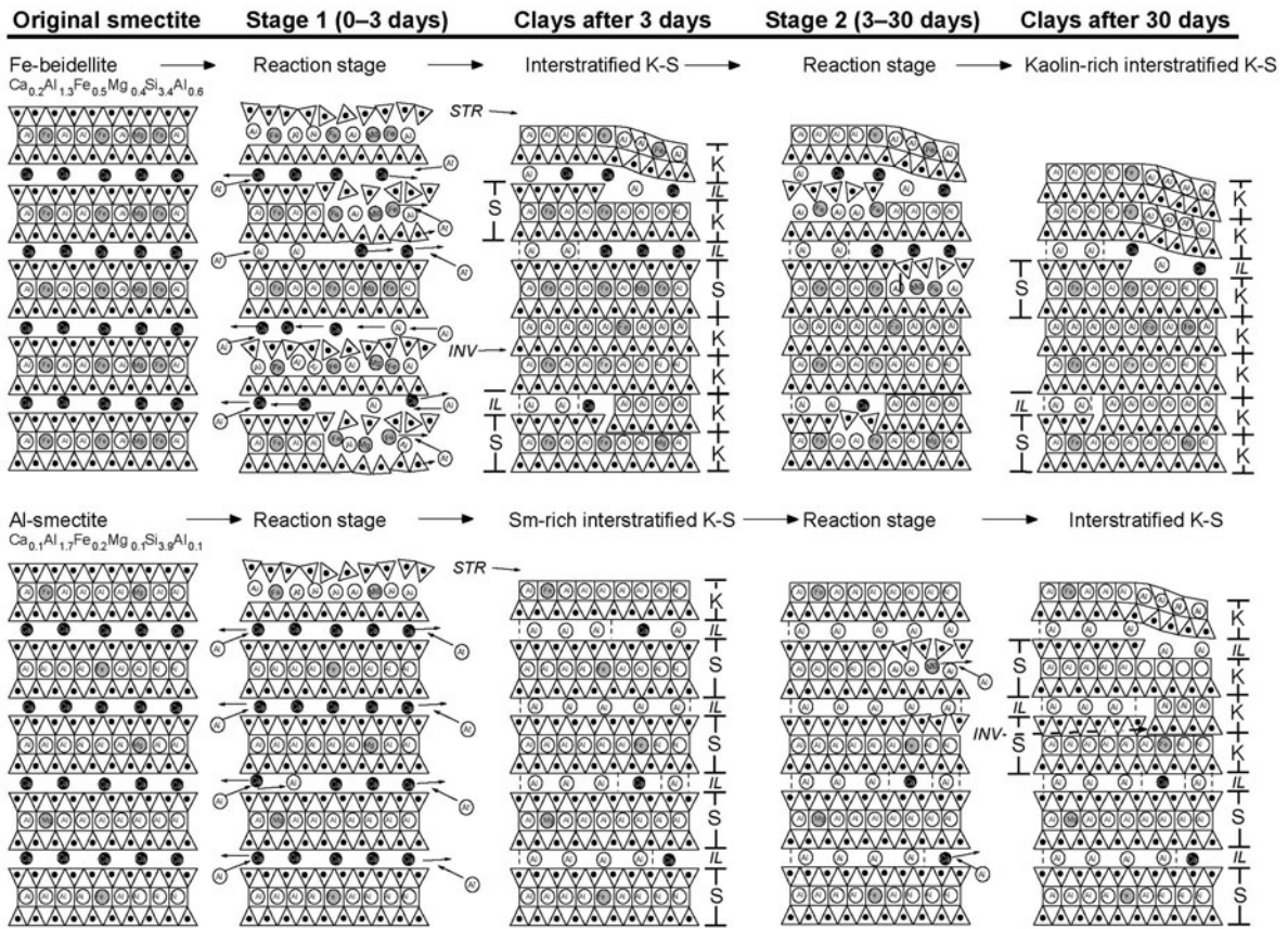
Figure 8. Interpreted reaction mechanisms of smectite layers to kaolinite layers emphasizing apparent differences in reaction rate between Fe-beidellite and Al-smectite end-members. In both examples, smectite layers transform to kaolinite layers laterally within crystals via tetrahedral stripping (STR) and tetrahedral inversion (INV). Smectite 2:1 layers and kaolinite 1:1 layers are denoted by S and K, and interlayers by IL, respectively. Black circles represent Ca^{2+} in interlayer sites; the occurrence of Al^{3+} in interlayers is also shown, where much interlayer Al occurs as Al-hydroxy complexes.
