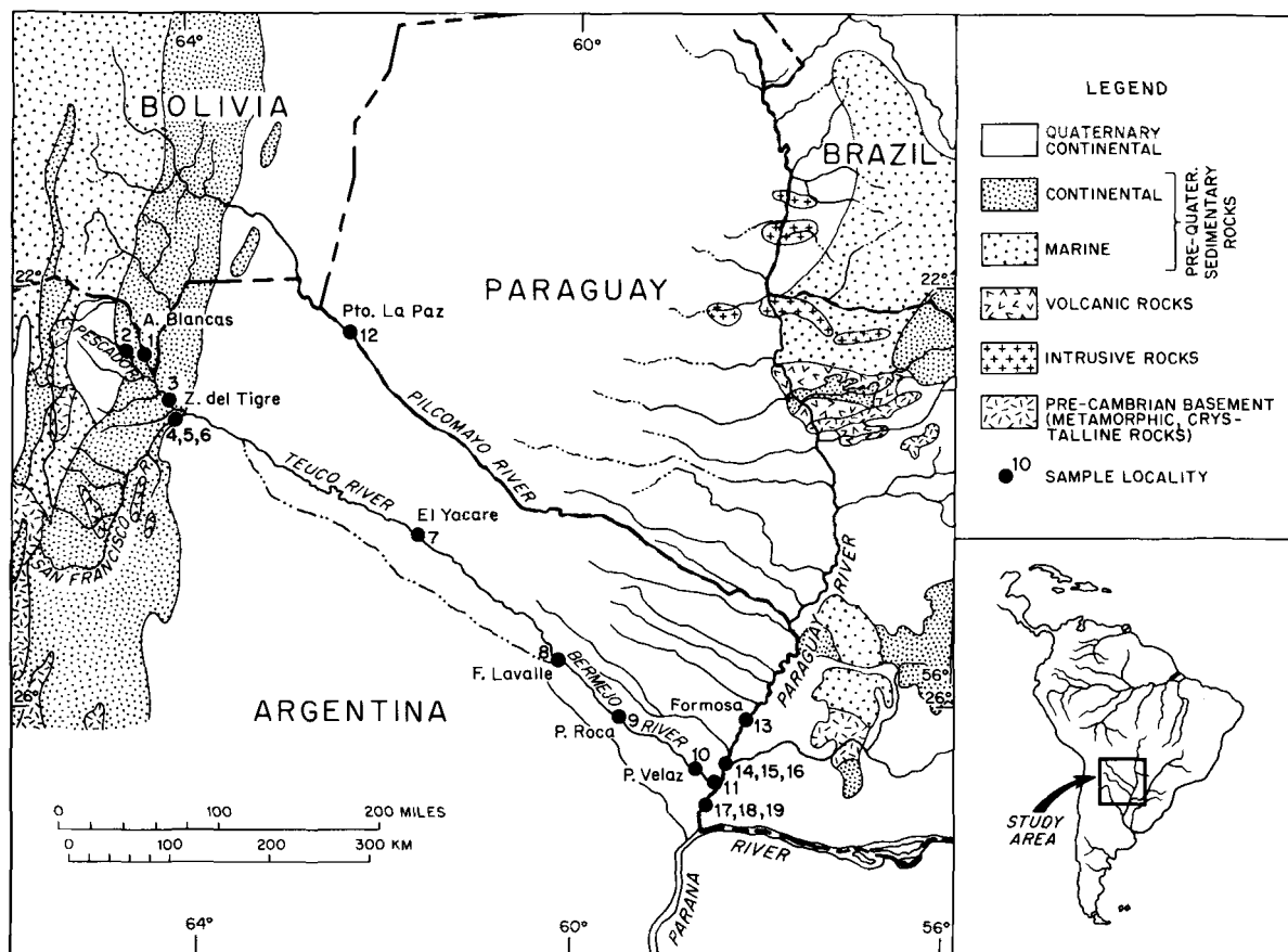
Figure 1. Schematic map showing the lithology of the area and the location of the samples.
