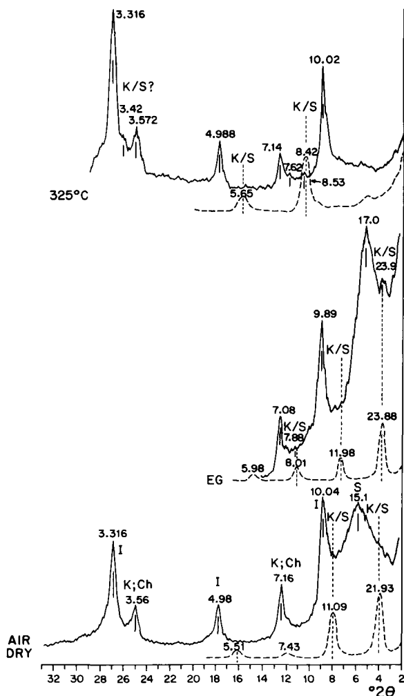
Figure 2. X-ray powder diffraction patterns (solid lines) of the natural sample and synthetic patterns generated with NEWMOD (dashed lines) for a kaolinite/smectite mineral. Synthetic patterns were provided by A. R. Thomas (Texaco Inc., 3901 Briar Park, Houston, Texas 77042).
