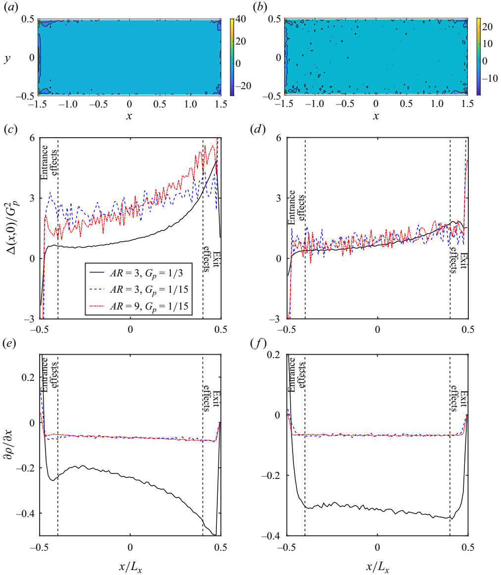
Figure 15. (a,b) Contours of the normalized dilatation ‘ \Delta(x, y)/G_p^2 ’ in the (x/L_y, y/L_y) -plane for G_p = 1/15 ( \delta p/p_0 = 0.2 ) and AR = 3 . (c,d) Axial variations of ‘ \Delta(x, 0)/G_p^2 ’ for three data sets: (i) black solid line ( G_p = 1/3 (i.e. \delta p/p_0 = 1.0 ) and AR = 3 ); (ii) blue dashed line ( G_p = 1/15 ( \delta p/p_0 = 0.2 ) and AR = 3 ); (iii) red dot-dashed line ( G_p = 1/15 ( \delta p/p_0 = 0.6 ) and AR = 9 ). (e,f) Axial variations of the density gradient ‘ \partial\rho(x, 0)/\partial x ’, with other parameters as in panels (c,d). The panels denote data for (a,c,e) Kn = 0.05 and (b,d,f) Kn = 0.5 , respectively. The wiggles seen in two data sets in (c,d) are due to (i) the discrete derivative calculations and (ii) the increased noise in the DSMC data at small values of G_p .
