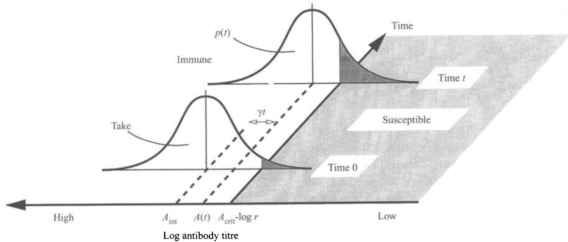
Fig. 1. A schematic overview of the model of antibody decay. Log antibody titres immediately after vaccination (time 0) are normally distributed around the mean A_{int} with variance \sigma^2 . Those cattle with log antibody titres above the threshold A_{crit} - \log r (where r is degree of homology) are protected (immune) and those with log antibody titres below the threshold are susceptible. Log antibody titre decays linearly through time at the rate \gamma so mean log antibody titre at time t is given by A(t) = A_{int} - \gamma t .
