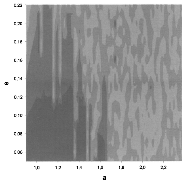
Fig. 3. Stability diagram of orbits in \gamma Cephei. The stability of orbits (initial semi-major axes of the fictitious planets (x-axis) versus initial eccentricity of the real planet (y-axis)) is labeled as follows: Black regions are orbits with e_f < 0.1 , dark grey regions e_f < 0.2 , light grey and white stand for orbits with eccentricities suffering sooner or later from close approaches to the massive planet and which are unstable.
