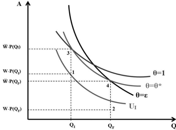
Figure 2. Consumption behaviour of formal-sector and informal-sector households.
