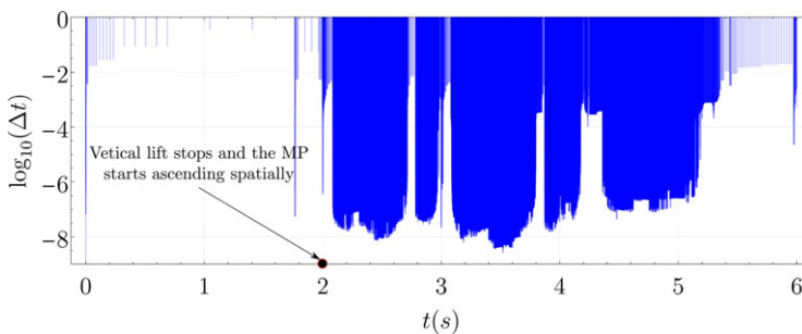
Figure 14. Variations in the step size \Delta t used by the solver ode15s at every instance of the simulation of the 4-4 CDRP for the input trajectories of the exit points of the cables b_k in Eq. (21). The sustenance of smaller steps can be seen during the spatial ascend and descend of the MP, that is, segments L_2 and L_3 in Fig. 7.
