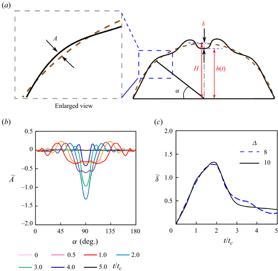
Figure 8. Deformation of the sessile droplet. (a) Schematic diagram showing capillary waves on the sessile droplet. The dashed brown line represents an undeformed droplet whereas the solid black line shows a deformed sessile droplet during the bouncing process. (b) Variation of normalized wave amplitude with angle \alpha at different time instants. (c) Evolution of normalized crater depth at the Z axis with time.
