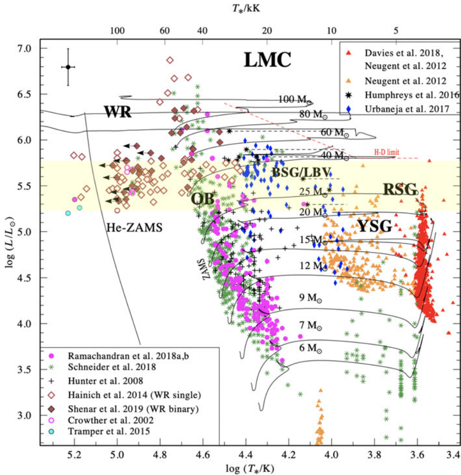
Figure 1. Various stellar populations (see legend) shown on a Hertzsprung-Russell diagram (HRD) of the LMC, adapted from Ramachandran et al. (2019) and Davies et al. (2018), Neugent et al. (2012), Humphreys et al. (2016), Urbaneja et al. (2017), Schneider et al. (2018), Shenar et al. (2019), Hainich et al. (2014), Crowther et al. (2002), Tramper et al. (2015), and Hunter et al. (2008). Tracks are single-star evolution tracks computed with the Modules for Experiments in Stellar Astrophysics (MESA) code (Paxton et al. 2011), taken from Gilkis et al. (2021). The WN population (which comprises roughly 80% of the total LMC WR population) is shown on the left part, with filled symbols depicting known binaries, and empty symbols depicting apparently-single WN stars. The WR population is not reproduced, notably the apparently-single stars. A similar picture is observed with other widely-used tracks, such as Geneva (Eggenberger et al. 2021) and BPASS (Eldridge & Stanway 2009, Eldridge et al. 2017). Highlighted is the overlap between cool supergiants and the WR populations, which includes only the most luminous cool supergiants. Figure courtesy of Varsha Ramachandran and Avishai Gilkis.
