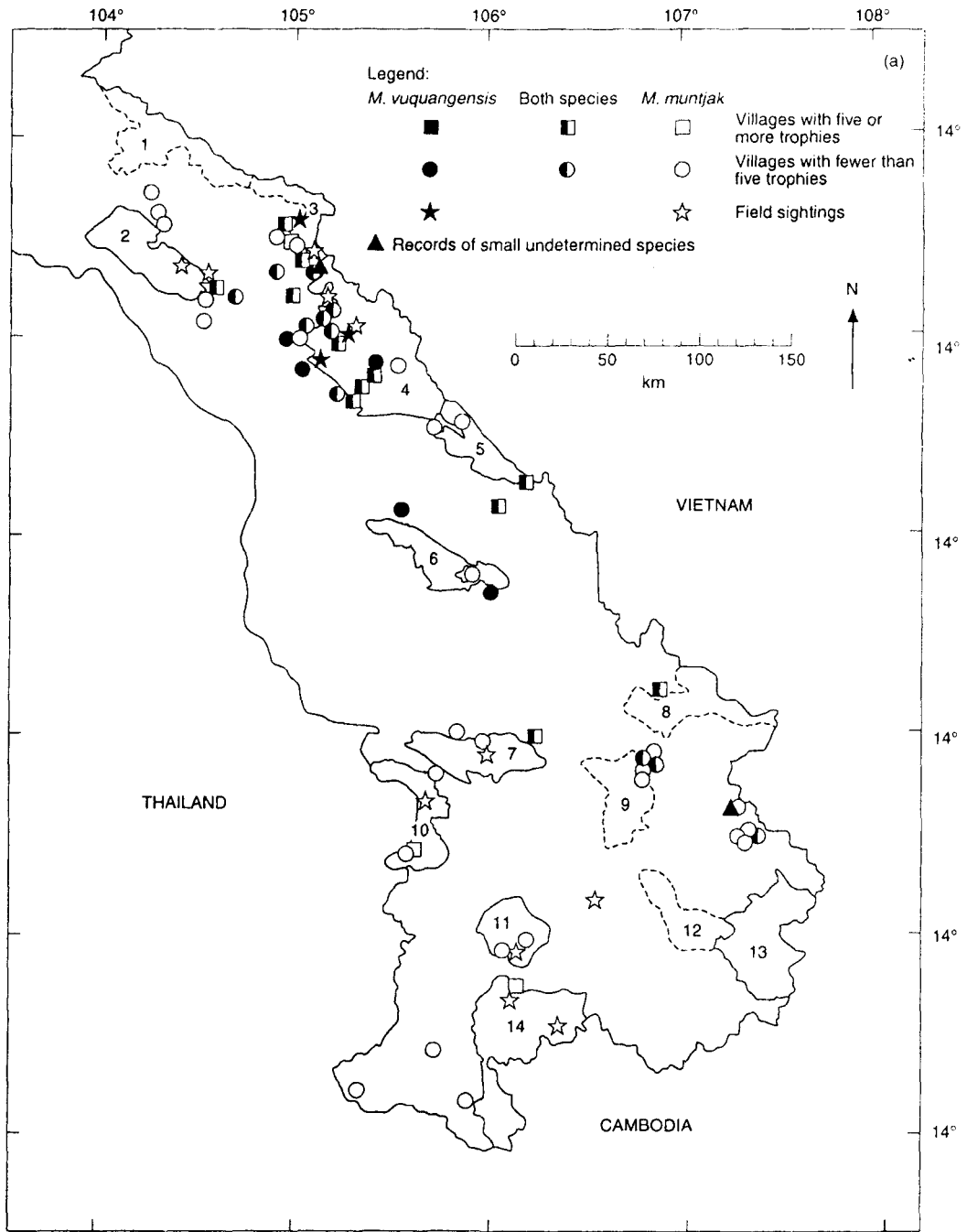
Figure 2(a). Central and southern Laos: protected areas and distributional records of Megamuntiacus vuquangensis and Muntiacus muntjak . National Biodiversity Conservation Areas and Proposed Protected Areas: 1, Nam Chuan PPA; 2, Nam Kading NBCA; 3, Nakai-Nam Theun proposed northern extension; 4, Nakai-Nam Theun NBCA; 5, Hin Namnu NBCA; 6, Phou Xang He NBCA; 7, Xe Bang Nouan NBCA; 8, Xe Sap PPA; 9, Phou Theung PPA; 10, Phou Xiang Thong NBCA; 11, Dong Hua Sao NBCA; 12, Phou Kathong PPA; 13, Dong Amphan NBCA; 14, Xe Pian NBCA
