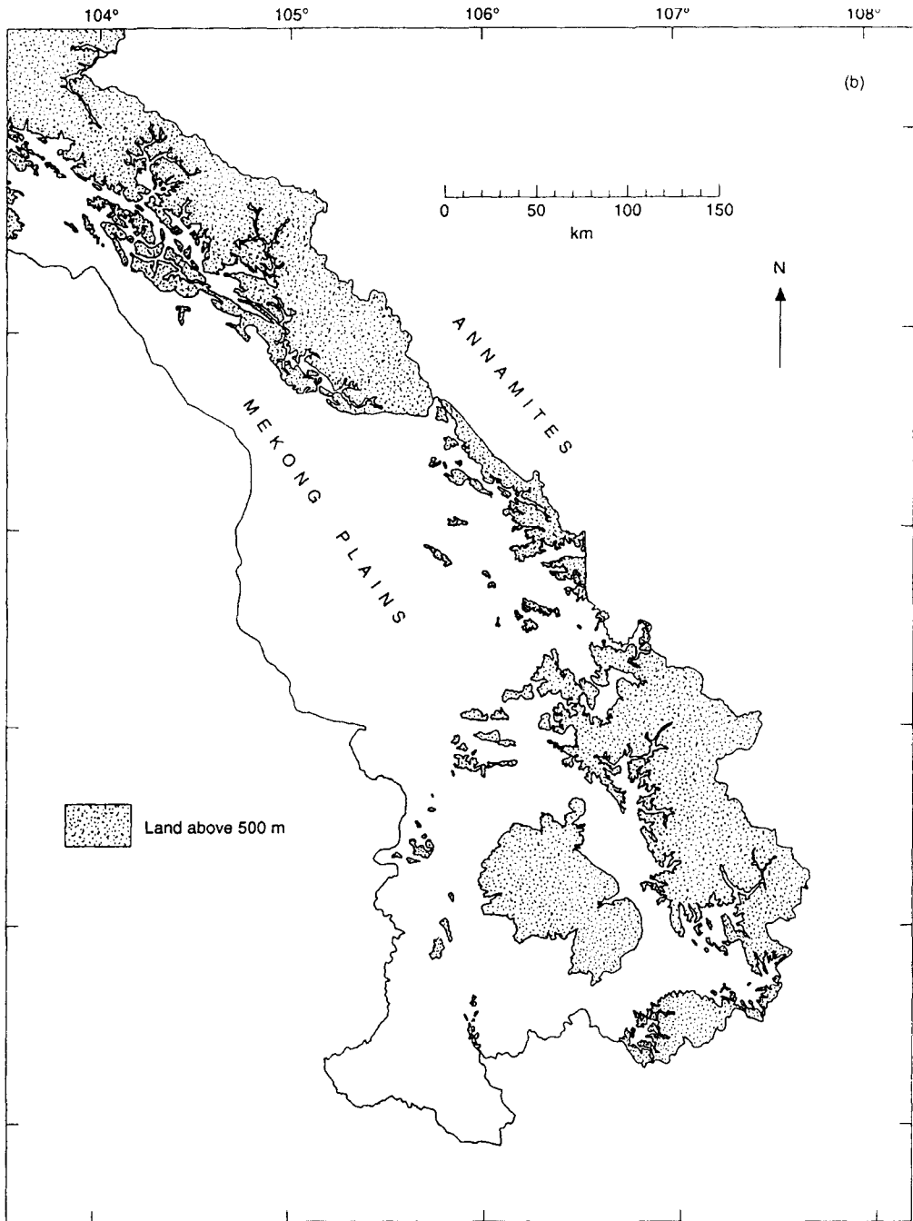
Figure 2(b). Central and southern Laos: the 500-m contour topographically delimiting the Annamite mountain and Mekong plains areas.
