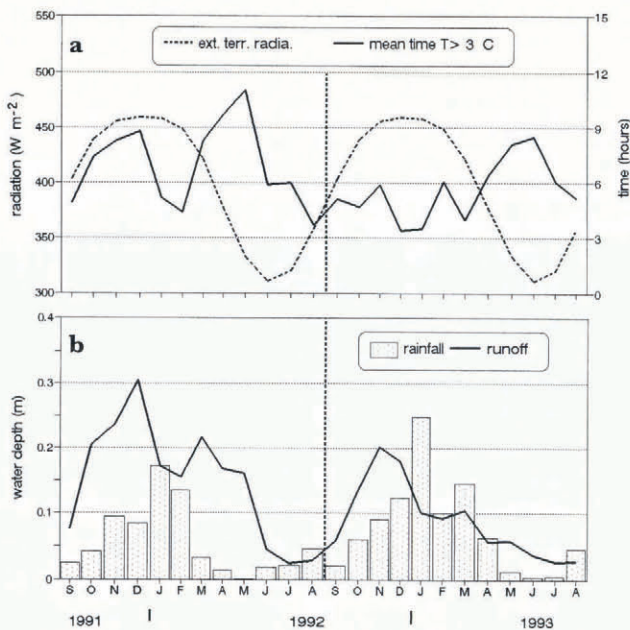
Fig. 6. (a) Extraterrestrial radiation and mean of hours per day with temperature above 3°C, and (b) rainfall and monthly runoff depth, on Zongo Glacier during the 2 years of the study.
