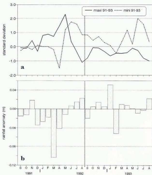
Fig. 2. Standard deviation of (a) maximum and minimum 1991–93 monthly temperatures from the 1953–93 mean at Chacaltaya (5230 m); (b) monthly 1991–93 precipitation from the 1972–93 mean at Plataforma Zongo (4770 m).
