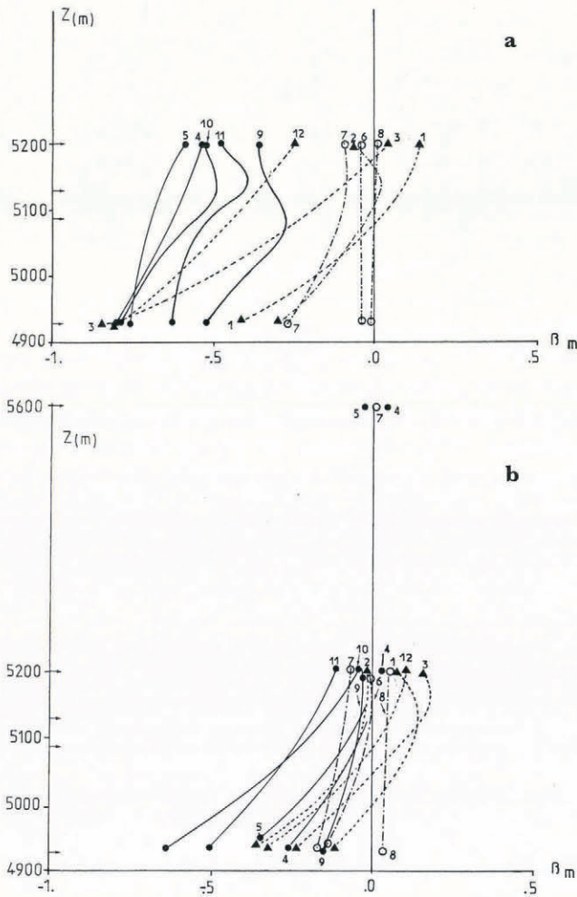
Fig. 4. Monthly net balance ( \beta_m in m of water) as a function of altitude ( Z ) during (a) 1991–92, and (b) 1992–93. Numbers 1–12 refer to the months. Solid line: September, October, November, April, May. Dashed line: June, July, August. Dotted line: December, January, February, March.
