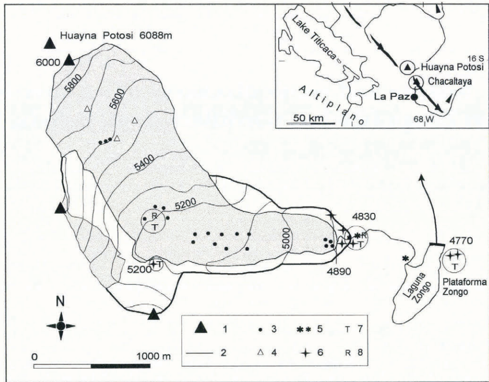
Fig. 1. Huayna Potosí and Zongo Glacier with the survey system in 1993. 1, Principal peaks; 2, Limits of basin; 3, Stakes; 4, Pits and crevasses; 5, Water-level recorder; 6, Rain-gauges; 7, Thermograph; 8, Pyranometer.
