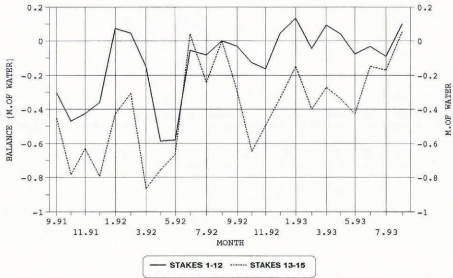
Fig. 3. Monthly balance from September 1991 to August 1993 in the ablation zone, calculated using two groups of stakes. Stakes 1–12 are situated near the ELA (5200–5100 m) and stakes 13–15 are near the glacier terminus (4900 m). The balance was estimated from a monthly stake reading and a density measurement of the snow/ice surface.
