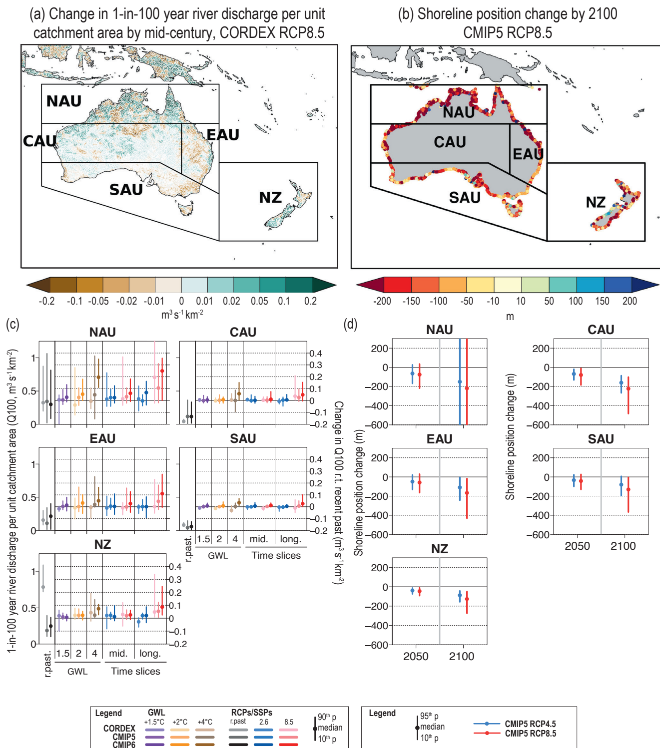
Figure 12.7 | Projected changes in selected climatic impact-driver indices for Australasia. (a) Mean change in 1-in-100-year river discharge per unit catchment area ( Q_{100} , \text{m}^3 \text{s}^{-1} \text{km}^{-2} ) from CORDEX-Australasia models for 2041–2060 relative to 1995–2014 for RCP8.5. (b) Shoreline position change along sandy coasts by the year 2100 relative to 2010 for RCP8.5 (metres; negative values indicate shoreline retreat) from the CMIP5-based dataset presented by Vousdoukas et al. (2020b). (c) Bar plots for Q_{100} ( \text{m}^3 \text{s}^{-1} \text{km}^{-2} ) averaged over land areas for the AR6 WGI Reference Regions (defined in Chapter 1). The left-hand column within each panel (associated with the left-hand y-axis) shows the 'recent past' (1995–2014) Q_{100} absolute values in grey shades. The other columns (associated with the right-hand y-axis) show the Q_{100} changes relative to the recent past values for two time periods ('mid' 2041–2060 and 'long' 2081–2100) and for three global warming levels (defined relative to the pre-industrial period 1850–1900): 1.5°C (purple), 2°C (yellow) and 4°C (brown). The bars show the median (dots) and the 10–90th percentile range of model ensemble values across each model ensemble. CMIP6 is shown by the darkest colours, CMIP5 by medium, and CORDEX by light. SSP5-8.5/RCP8.5 is shown in red and SSP1-2.6/RCP2.6 in blue. (d) Bar plots for shoreline position change along sandy coasts for 2050 and 2100 relative to 2010 for RCP8.5 (red) and RCP4.5 (blue) from Vousdoukas et al. (2020b). Dots indicate regional mean change estimates and bars show the 5–95th percentile range of associated uncertainty. Note that these shoreline position change projections assume that there are no additional sediment sinks/sources or any physical barriers to shoreline retreat. See Technical Annex VI for details of indices. Further details on data sources and processing are available in the chapter data table (Table 12.SM.1).
