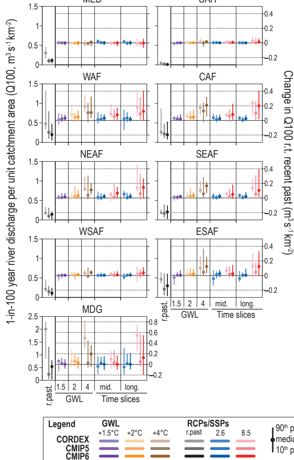
Figure 12.5 | Projected changes in selected climatic impact-driver indices for Africa.
