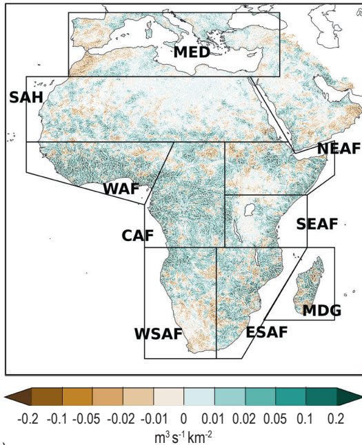
(a) Change in 1-in-100 year river discharge per unit catchment area by mid-century, CORDEX RCP8.5
