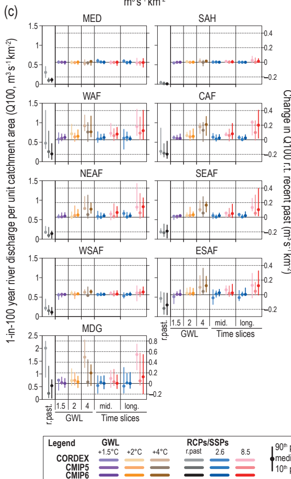
Figure 12.5 | Projected changes in selected climatic impact-driver indices for Africa.
