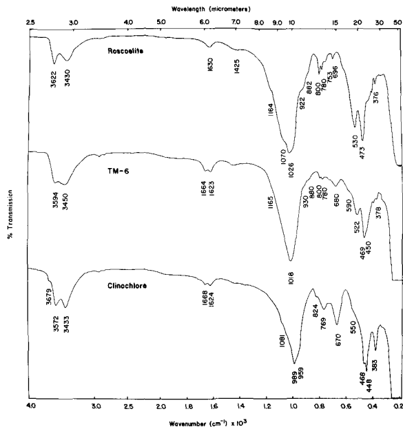
Figure 6. Infrared spectra for roscoelite (Rifle, Colorado) (upper spectrum), vanadium chlorite sample TM6 (middle spectrum), and clinocllore (Silver Peak, Montana) (bottom spectrum). Absorption bands are labeled in wave numbers.
