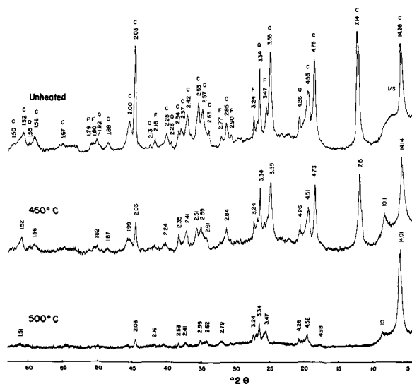
Figure 4. X-ray powder diffraction patterns for unheated and heated vanadium chlorite sample TM6. All patterns are for random powder mounts; peak labels are in Å.
