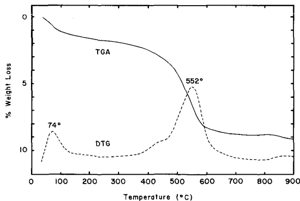
Figure 5. Thermogravimetric data for vanadium chlorite sample TM6. The upper curve (TGA) registers percent weight loss and the bottom curve (DTG) is the differential thermogravimetric curve which indicates points of maximum rate of weight loss.
