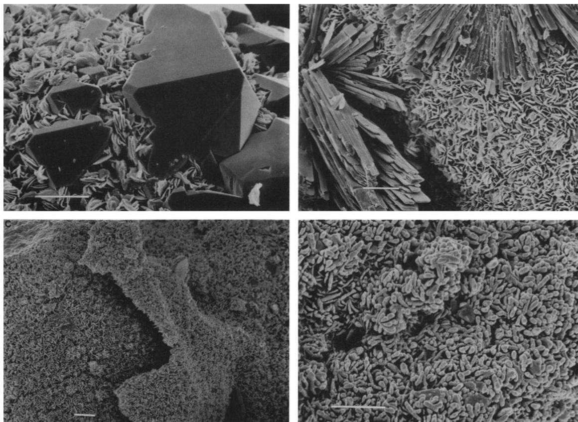
Figure 3. Textures of authigenic minerals. (A) Thin-flake chlorite with overgrowths of quartz. (B) House-of-cards vanadium chlorite with fan-shaped vanadium oxide crystals overgrowing it. (C) A layer of rounded-flake vanadium chlorite on top of the thin-flake house-of-cards vanadium chlorite. (D) Closer view of the rounded-flake vanadium chlorite. Bar scale on each photo is 10 \mu\text{m} .
