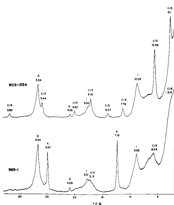
Figure 2. X-ray powder diffraction patterns for two mixed-layer chlorite/smectites. Sample WC6-1554 (top) is from sandstone adjacent to, and immediately below the most strongly mineralized zone. The chlorite/smectite is dioctahedral and is sufficiently well ordered to be called tosudite. Sample 969-1 is from an ore zone which has been exposed to oxidizing conditions and probably represents the degradation product of vanadium chlorite. C/S = mixed-layer chlorite/smectite; I = illite; K = kaolinite; Q = quartz. Both samples are the <2\text{-}\mu\text{m} fraction and were X-rayed using \text{CuK}\alpha radiation.
