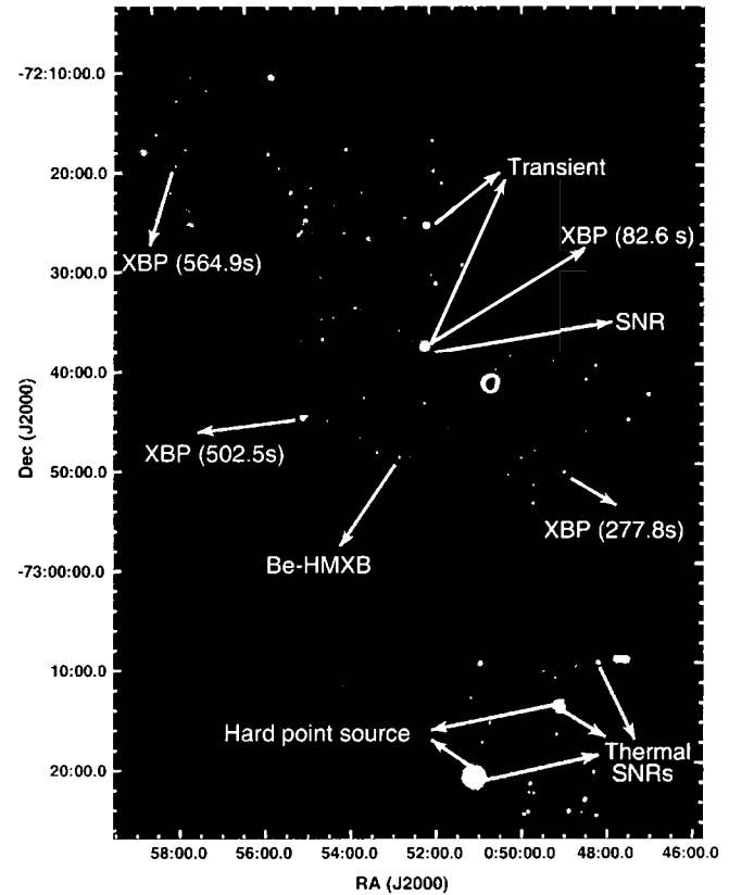
Fig. 1. A full band (0.5–7.5 keV) adaptively smoothed, exposure corrected image of the 5 Chandra fields showing a few examples of identified pulsars, transient sources and SNRs.
