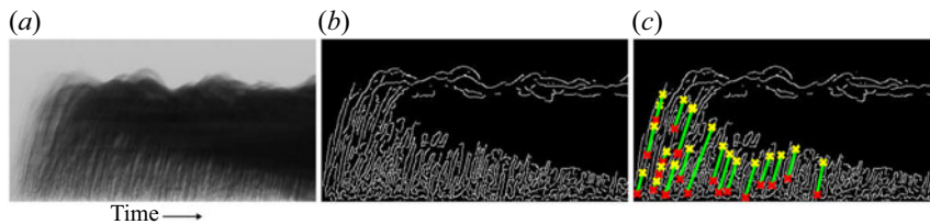
Figure 13. Procedure used to estimate the speed of the rising fountain flow in our experiments. (a) Grey scale centreline time series showing rising fountain mixture (forward-sloping lines), (b) output of the edge detection function in Matlab and (c) output of Hough transform used to calculate the gradient of the forward-sloping lines in the time series.
