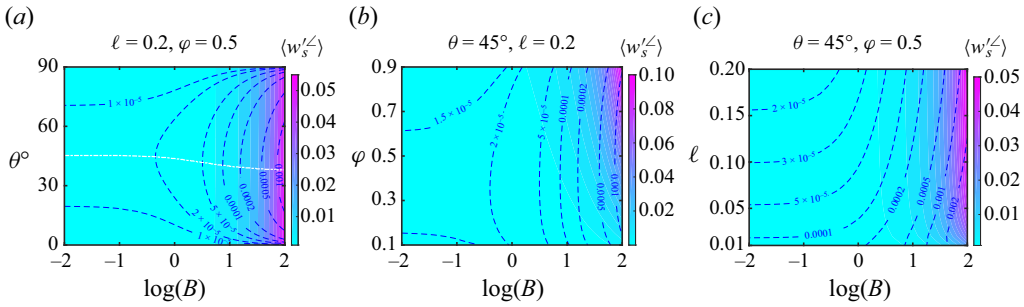
Figure 8. Variations of averaged main ( \langle w'_s \rangle ) and secondary ( \langle u'_s \rangle ) slip velocities vs (a) \theta and B , (b) \varphi and B and (c) \ell and B , at b = 0.001 . Colours represent data for the main slip component ( \langle w'_s \rangle ), whereas blue dashed lines show those of the secondary flow component ( \langle u'_s \rangle ). The white dash-dotted line in panel (a) shows the \theta value at which the maximum of secondary flow slip component occurs.
