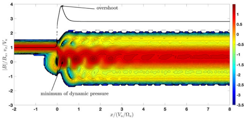
FIGURE 4. Reduced 1-D distribution f(x, v_x) , together with the magnetic profile.
