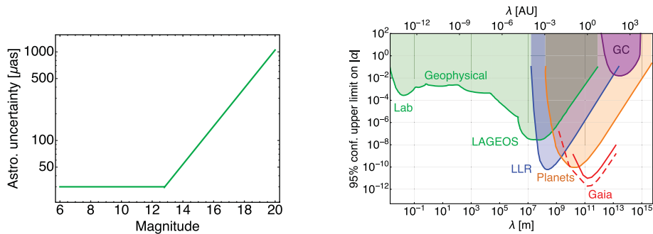
Figure 1. Left: astrometric uncertainty of SSOs observations as a function of the magnitude. Right: Existing constraints on the fifth force parameters. The solid Gaia curve corresponds to constraint reachable using 5 years of SSOs observations with Gaia while the dashed Gaia line corresponds to an extended mission.
