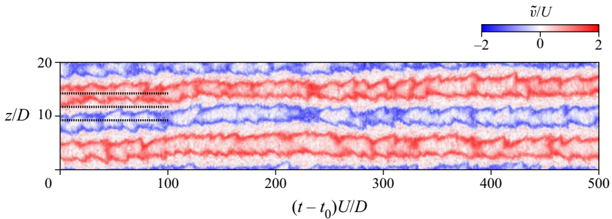
Figure 19. Spacetime diagram of the low-pass filtered crossflow velocity at the location (x/D, y/D) = (2, 0) over the time interval 0 \leq (t - t_0)U/D \leq 500 for Re = 3900 . The dotted lines indicate the locations and time interval where local flow statistics are taken.
