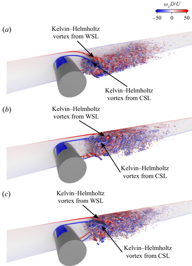
Figure 13. Contours of the spanwise vorticity for the case of Re = 3900 as in figure 12. Overlain are isosurfaces of \lambda_2 = -15 between (a) 9.5 \leq z/D \leq 10.5 , (b) 12 \leq z/D \leq 13 and (c) 14.5 \leq z/D \leq 15.5 . Isosurfaces are colourised by the spanwise vorticity.
