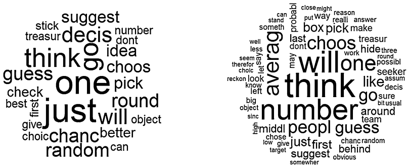
(a) Level-0. T = 58 , \sum_t x_t = 181 , x_{\text{just}} = 12 .
