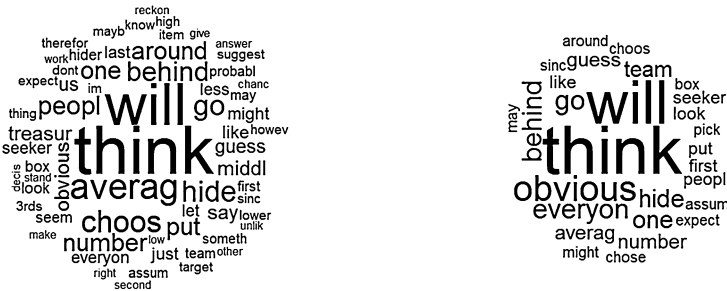
(c) Level-2. T = 92 , \sum_t x_t = 568 , x_{\text{think}} = 50 .
