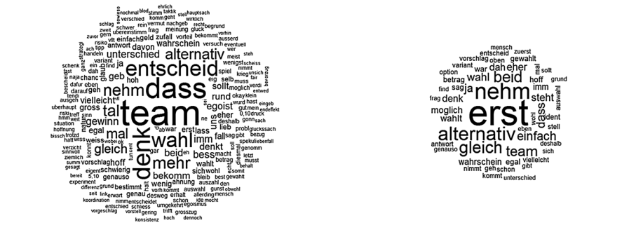
(a) No label salience (none, X-Y games). T = 275, \sum_t x_t = 3069, x_{team} = 194.
