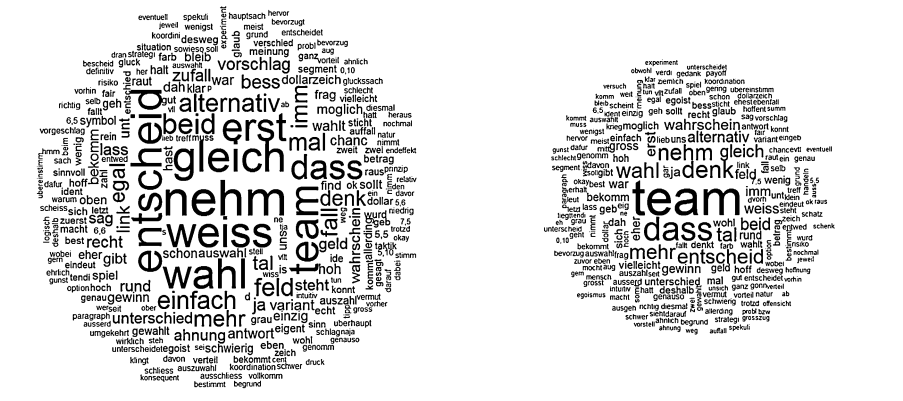
(a) Level-0. T = 295, \sum_t x_t = 2601, x_{\text{nehm}} = 83. (b) Level-1. T = 294, \sum_t x_t = 2731, x_{\text{team}} = 196.
