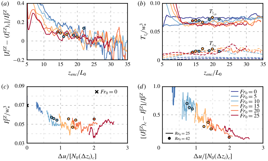
FIGURE 13. (Colour online) Temporal evolution of the contributions from the accumulation term, I_t^{EZ} , and the turbulent-transport term, I_T^{EZ} = T_{z_i,0} - T_{z_\infty} , to the TKE budget equation (5.1). The subscript c indicates the convective limit Fr_0 = 0 .
