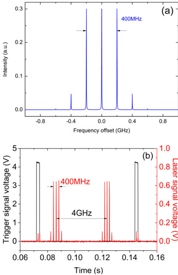
Figure 2. (a) Simulated spectra and (b) experimental spectra of phase-modulated triple-frequency seed laser.
