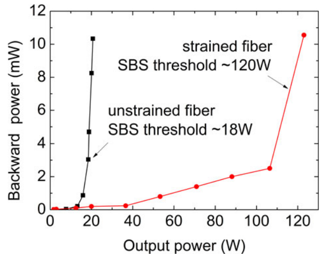
Figure 4. Backward power as a function of the output power.
