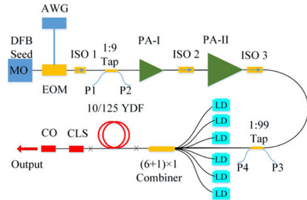
Figure 1. Experimental setup of monolithic fiber amplifier system (MO: master oscillator; PA, pre-amplifier; CO, collimator).
