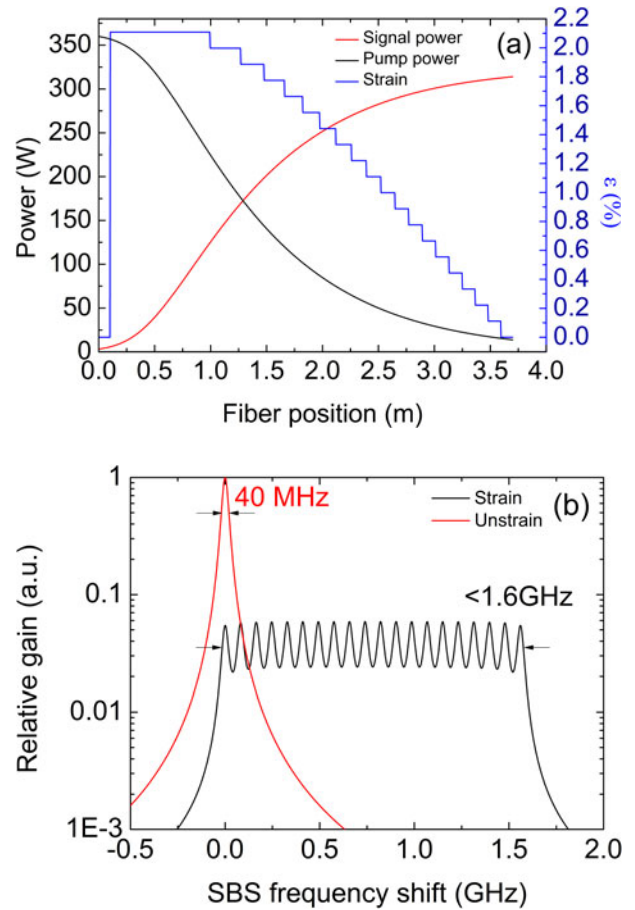
Figure 3. (a) Strain distribution along the active fiber. (b) SBS gain spectra of strained and unstrained fiber.
