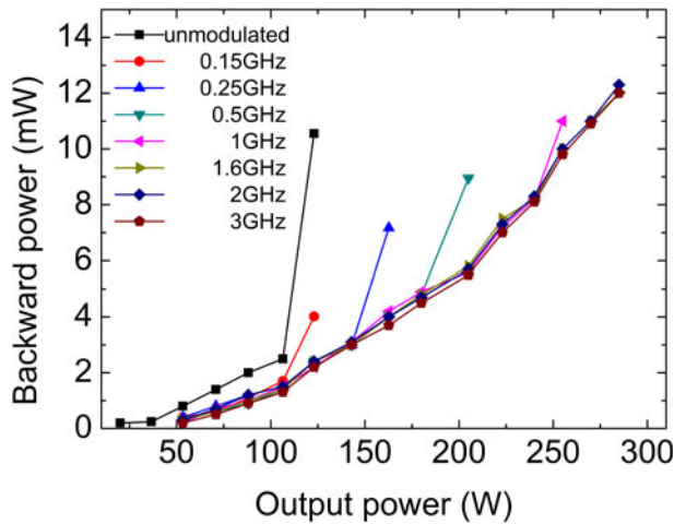
Figure 6. Backward power as a function of the output power with different modulated frequencies.
