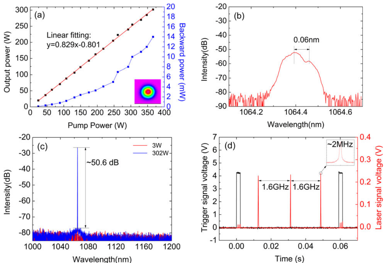
Figure 7. (a) Output power and backscattering power versus pump power. (b) Emission spectra of backward scattering. (c) Emission spectra of forward output laser. (d) FPI scanning spectra of triple frequency at the maximum output power.
