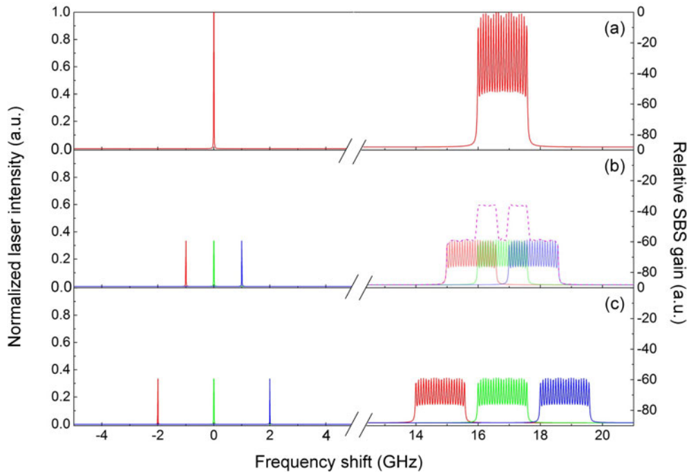
Figure 5. Overlap of the SBS gain spectra (a) without the modulation frequency; (b) with the modulation frequency of 1 GHz; (c) with the modulation frequency of 2 GHz [the short dashed line in (b) represents envelope of the total SBS gain].
