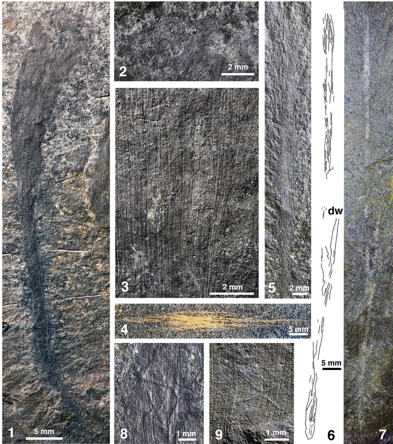
Figure 3. (1–7) Leptomitus zitteli Walcott, 1886. (1–3) USNM 15308, lectotype, entire specimen, plumose spicules evident at distal termination, long vertical and short horizontal oxeas. (4) YPM IP 543326, isolated bunch of oxeas. (5–7) YPM IP 239151, distal end showing long vertical oxeas, explanatory drawing of entire specimen (dw = detached wall), and entire specimen showing apparent branching. (8, 9) Protospongia hicksi Hinde, 1887, isolated cruciform spicules associated with USNM 15308, and associated with USNM 419731.
