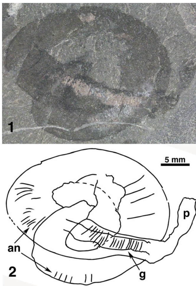
Figure 4. ? Ottoia Walcott, 1911 (Walcott, 1911b), (1, 2) YPM IP 239053, specimen and explanatory drawing. an = trunk annulations; g = gut trace; p = proboscis.
