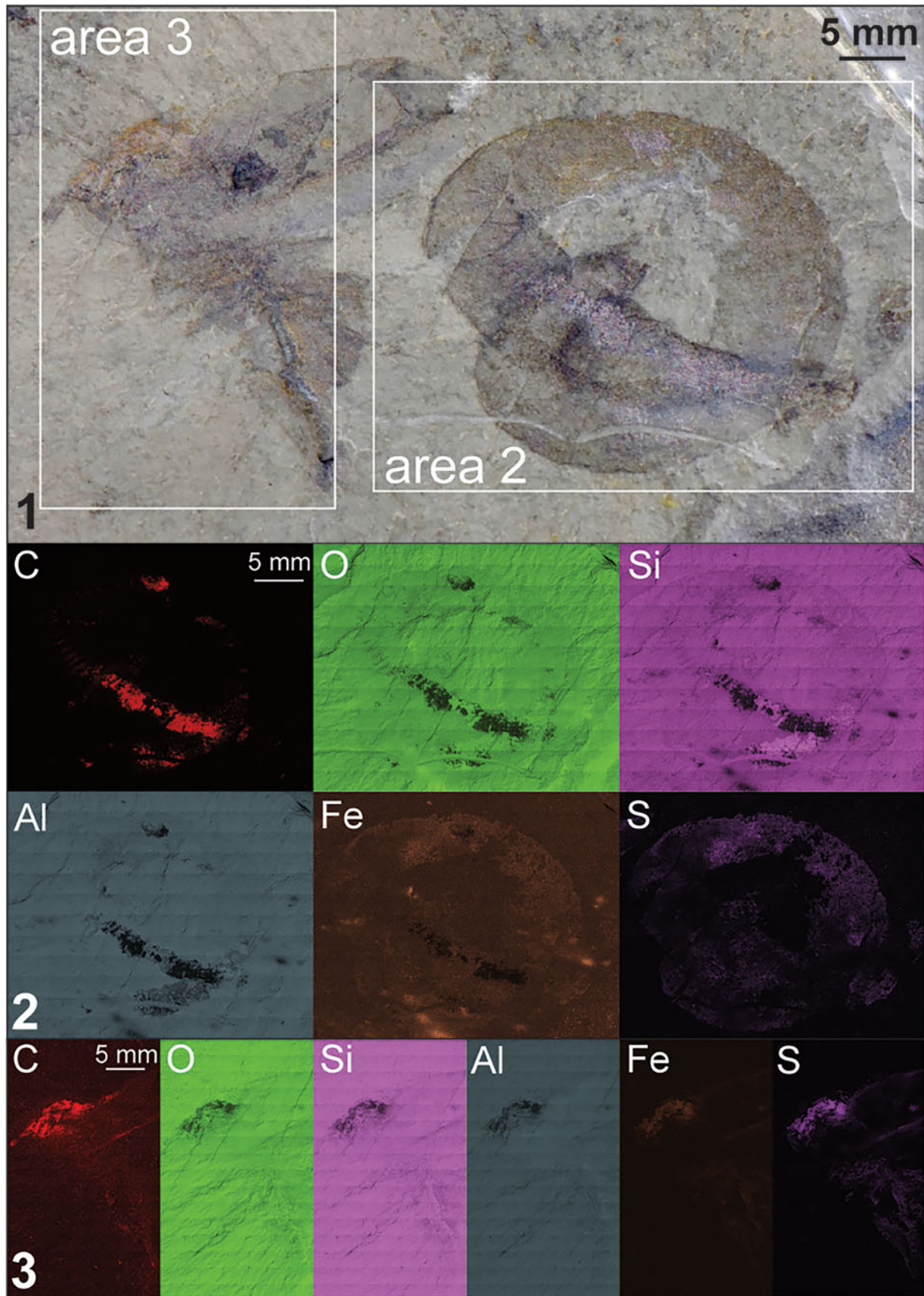
Figure 1. EDS elemental maps of Otoia (YPM IP 239053) and Vermontcaris montcalmi n. gen. n. sp. (YPM IP 543321). (1) Photograph of YPM IP 239053 and YPM IP 543321, showing the areas mapped. (2, 3) Elemental maps showing the distribution of C, O, Al, Si, Fe, and S in areas (2) (YPM IP 239053) and (3) (YPM IP 543321).
