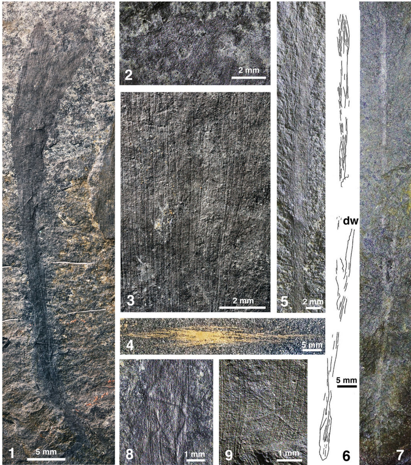
Figure 3. (1–7) Leptomitus zitteli Walcott, 1886. (1–3) USNM 15308, lectotype, entire specimen, plumose spicules evident at distal termination, long vertical and short horizontal oxes. (4) YPM IP 543326, isolated bunch of oxes. (5–7) YPM IP 239151, distal end showing long vertical oxes, explanatory drawing of entire specimen (dw = detached wall), and entire specimen showing apparent branching. (8, 9) ?Protospongia hicksi Hinde, 1887, isolated cruciform spicules associated with USNM 15308, and associated with USNM 419731.
