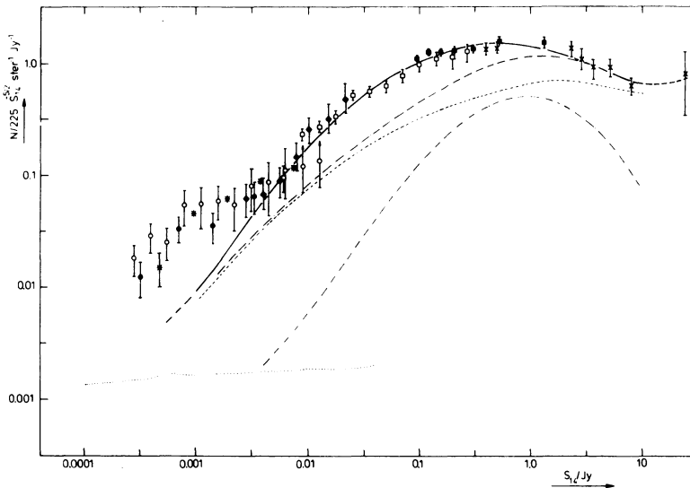
Figure 1. The 1.4 GHz differential source count normalized to a differential Euclidean count ( 225 S^{-5/2} \text{Sr}^{-1} \text{Jy}^{-1} ). References to older data ( S \geq 10 mJy) can be found in Willis et al. (1977). Filled circles: Condon and Mitchell (1982), open circles: Windhorst et al. (1983 5\sigma sample, asterisks: Windhorst et al. 6.5\sigma sample, - . - : observed count of radio-loud quasars, ----: count of powerful radio ellipticals out to z \sim 0.85 , calculated from observed RLF, and assuming non-evolving RLF below \log P \sim 25.0 , -.-: sum of two above, —: total count of quasars and powerful ellipticals, with elliptical RLF extrapolated out to z \sim 1.5 (as described in text), and again assuming no evolution below \log P \sim 25.0 .
