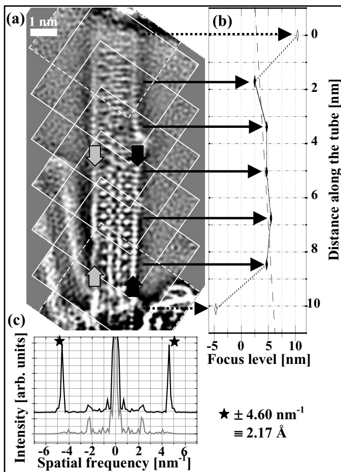
FIG. 1. (a) Restored phase of the imaged encapsulation composite ' \text{LaI}_2@(\text{18,3})\text{SWNT} ', obtained by recombination of six individually restored subregions (white frames). (b) Plot of the defocus value of each subregion versus its centre displacement along the tube axis. (c) Power spectra of line profiles along each of the SWNT walls, indicated by the arrows in Figure 1(a).
