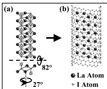
FIG. 3. (a) Modelled fragment of a {100} layer of bulk \text{LaI}_3 ; the iodine atoms missing in the images system are indicated with crosses. (b) Structural model of the proposed \text{LaI}_2@(\text{18,3})\text{SWNT} (upper SWNT wall omitted for clarity).
