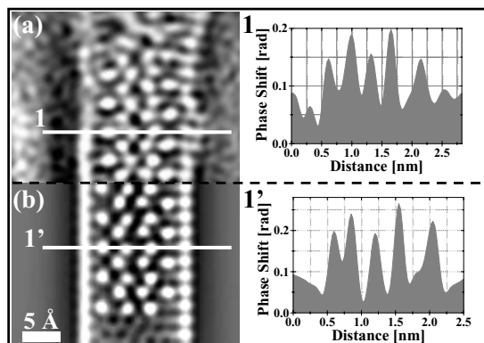
FIG. 2. (a) Selected region of the restored phase, shown in Figure 1(a). (b) Simulated \text{LaI}_2@(\text{18,3})\text{SWNT} composite. The white lines in Figures (a) and (b) indicate the single-pixel line traces displayed in diagrams (1) and (1') respectively.
