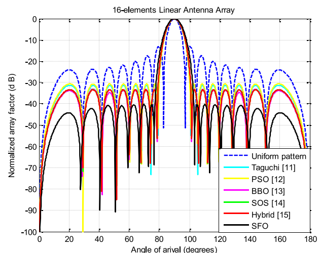
Figure 6. Radiation patterns of 16-element LAA.
