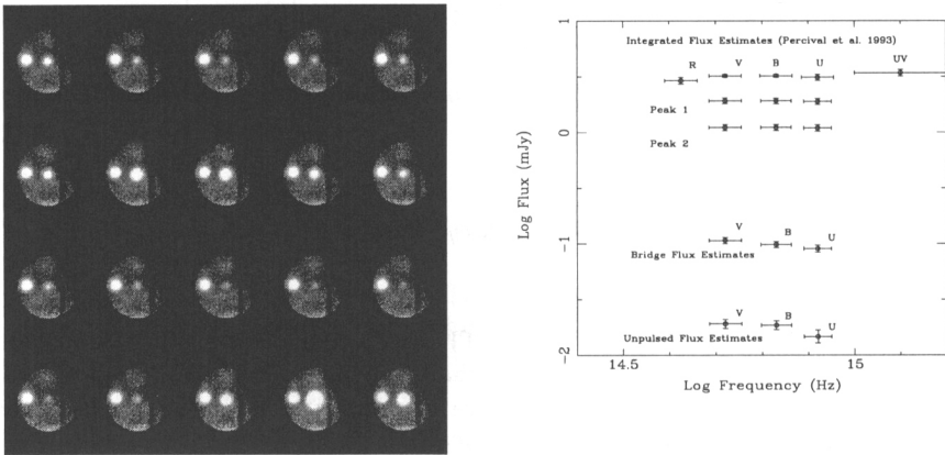
Figure 1. Left: Mosaic image of one full cycle of the Crab pulsar, via phase-resolved photometric analysis. The light curve moves from top left to bottom right. Note the ‘on’ emission throughout. Right: Integrated de-extinguished flux estimates for the Crab from Percival et al. 1993 and the derived flux estimates for both the peaks, Bridge and unpulsed component of emission based on the TRIFFID datasets.
