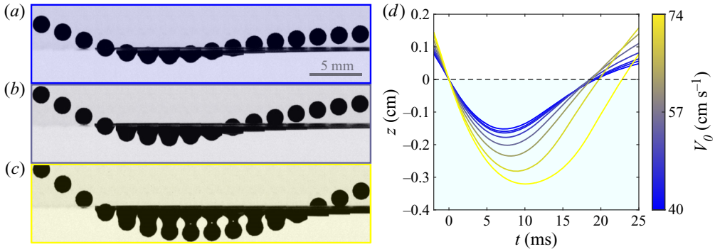
Figure 2. Rebound data for superhydrophobic spheres with radius R_s = 0.083 \text{ cm} and density \rho_s = 2.2 \text{ g cm}^{-3} . (a–c) Sequence of images of spheres with different impact speeds V_0 : (a) 40.2 \pm 0.7 \text{ cm s}^{-1} , (b) 53.7 \pm 0.7 \text{ cm s}^{-1} , (c) 73.6 \pm 0.6 \text{ cm s}^{-1} . Images are evenly spaced in time by 2 ms, corresponding to 20 frames. (d) Trajectories of the bottom of the spheres (relative to the undisturbed free-surface height) measured for eight different impact velocities. Shown are the average trajectories over all trials at a fixed release height with outliers removed, as described in the text. Videos corresponding to the trials shown in (a–c) are available as supplementary material at https://doi.org/10.1017/jfm.2020.1135 .
