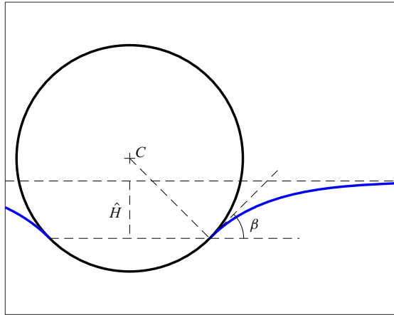
Figure 13. Schematic diagram for the quasi-static analysis. Point C corresponds to the centre of the sphere, \hat{H} is the depth of the boundary of the contact line and \beta is the angle formed between the horizontal and the free surface, where it meets the solid.
