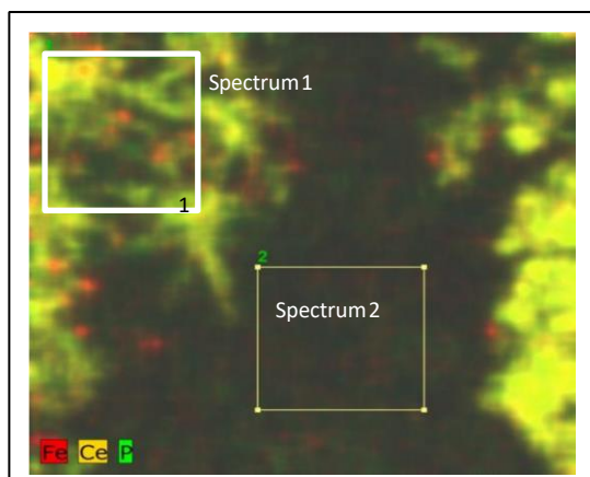
Figure 2. (Upper) EDS spectra of selected areas show distinct elemental content in location 1 (in green) and location 2 (in red); (lower) elemental maps showing distribution of elements Ce (yellow) and P (green) which correspond to cerium phosphate nanoneedles and Fe (red) which marks the location of ferritin nanoparticles.
