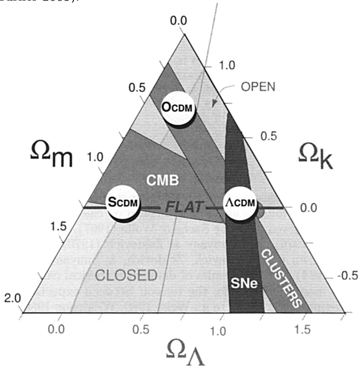
Figure 1. The Cosmic Triangle from Bahcall et al. (1999). This shows the concordance model for cosmological observations at the end of the last millennium. Three different classes of observations, supernovae, clusters, and CMB anisotropy, are consistent if we live in a spatially flat universe with a cosmological constant.
