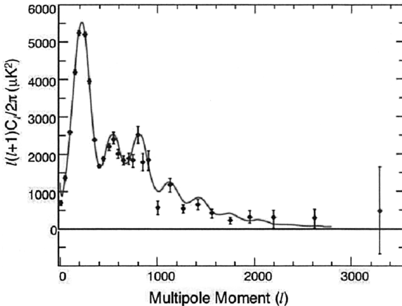
Figure 2. The Grand Unified Spectrum based on Bond, Contaldi, & Pogosyan (2003). The y axis shows the fluctuation power per logarithmic interval in l . The x-axis may be converted to angular scale by \theta_{deg} = l/200 . This spectrum is derived from the combination of 28 anisotropy experiments as of July 2003. The first and second peaks from the acoustic oscillations are clearly evident, the third peak is almost resolved, and the damping tail at l > 1000 is evident. The line is the best fit model.
