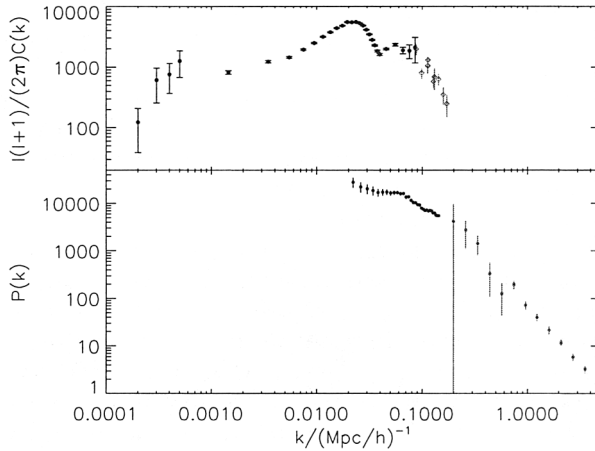
Figure 5. Top: the CMB angular power spectrum as a function of comoving wavenumber k ( k \approx l/14400 ). The points to the left are from WMAP , the data for l > 875 are from CBI and ACBAR. Bottom: the LSS data from 2dFGRS ( 0.01 < k < 0.15 ) and the Lyman \alpha survey (Croft et al. 2002). The power spectra have been rescaled to z = 0 . To compare the LSS data to the CMB one must take into account redshift-space distortions, non-linearities, bias, window functions, etc. This figure from Verde et al. (2003)
