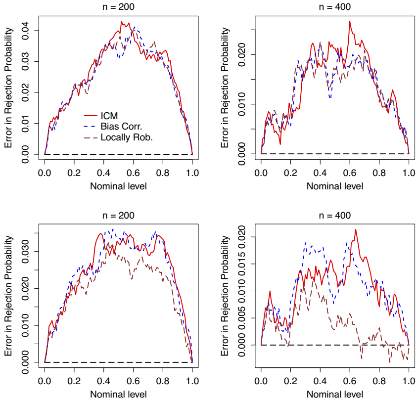
FIGURE 2. Errors in rejection probabilities using a data-driven bandwidth: results with trimming on first row, results with no trimming on second row.
