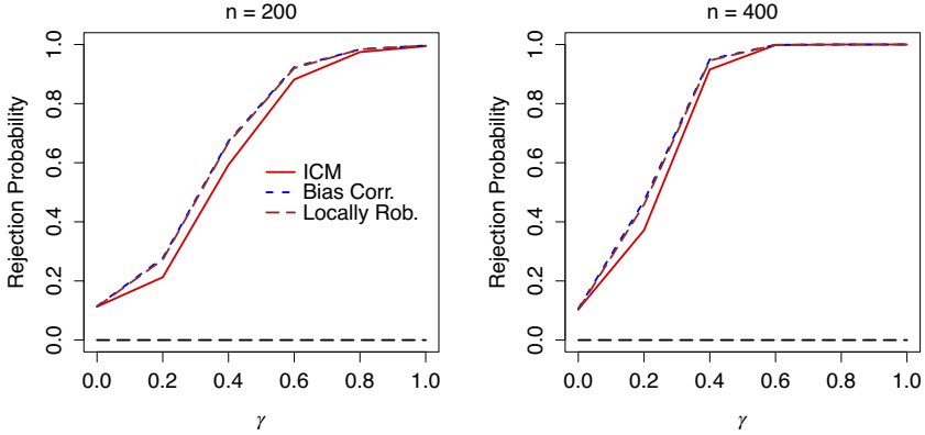
FIGURE 3. Power curves for tests at 10% level using a data-driven bandwidth and no trimming.
