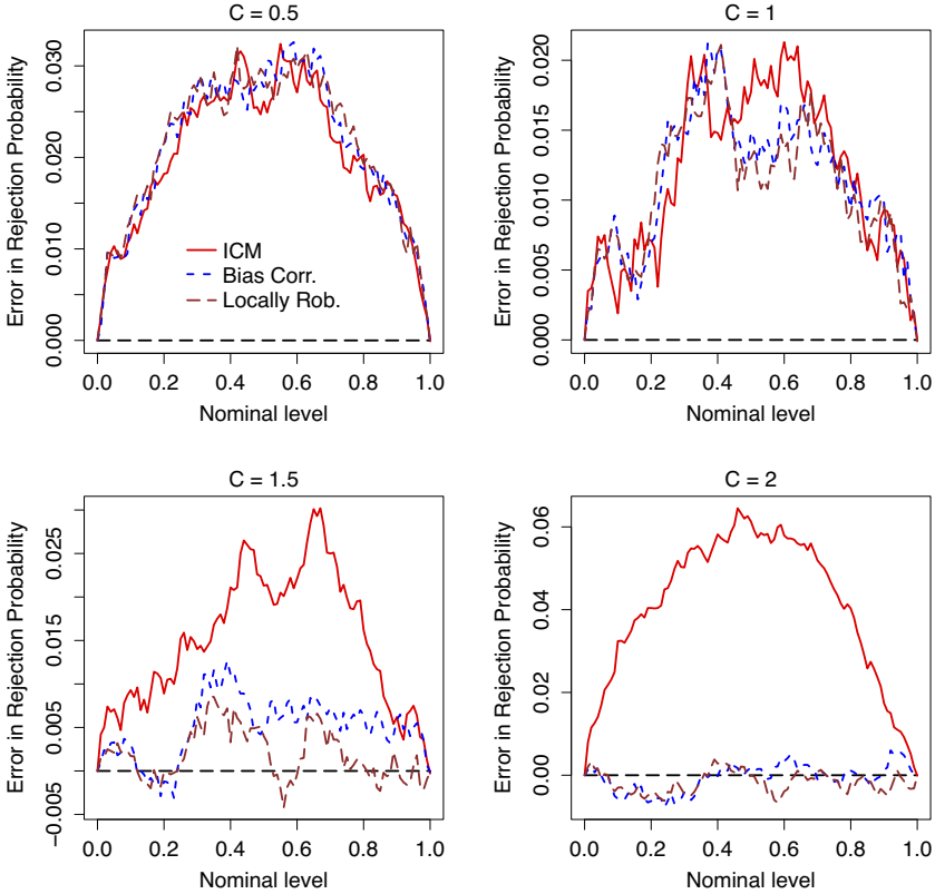
FIGURE 1. Errors in rejection probabilities for n = 400 using a rule-of-thumb bandwidth h = C\hat{\sigma}_W n^{-1/5} .
