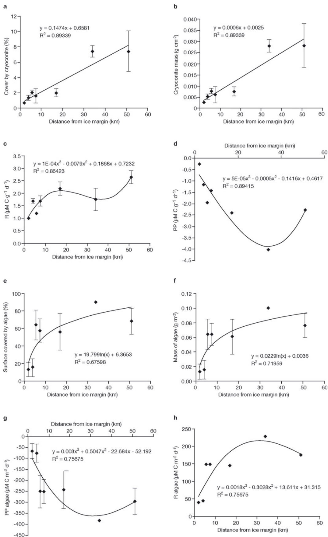
Fig. 3. (a) Percentage of ice surface covered by cryoconite with distance from ice margin (linear fit shown); (b) mass of cryoconite per square centimetre with distance from ice margin (linear fit shown); (c) respiration rates for cryoconite with distance from ice margin (third-order polynomial fit shown); (d) rate of primary production for cryoconite with distance from ice margin (no error bars because PP was calculated directly from NEP and R; third-order polynomial fit shown); (e) percentage cover of ice surface by surficial algae with distance from ice margin (logarithmic fit shown); (f) mass of algae per square metre with distance from ice margin (logarithmic fit shown); (g) primary production of surface algae against distance from ice margin (third-order polynomial fit shown); (h) respiration rate for surface algae against distance from ice margin (no error bars as this was assumed to be a constant proportion of algal PP; third-order polynomial fit shown).
