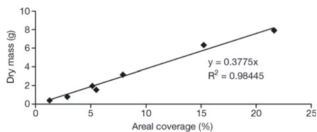
Fig. 2. Relationship between areal coverage and dry mass for calibration quadrats. Note that calibration quadrats refer to 10 \text{ cm} \times 10 \text{ cm} quadrats emplaced at the 2 km site for which the mass of cryoconite present was measured, not the 81 test quadrats emplaced along the transect.
