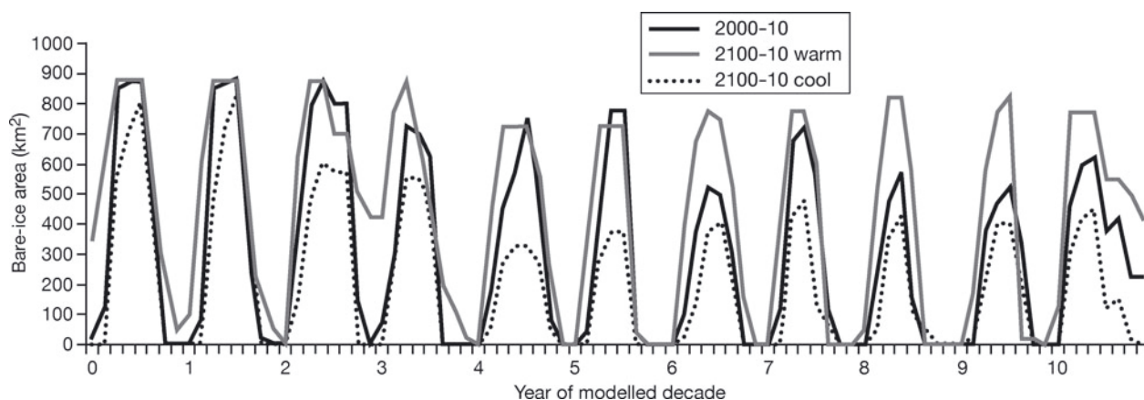
Fig. 8. Bare-ice areas as predicted by the warm GrIS, cool GrIS and present-day simulations.
