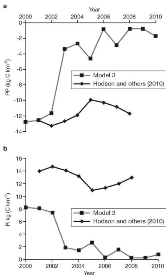
Fig. 6. (a) Carbon flux resulting from cryoconite community autotrophy as predicted by model 3 and Hodson and others (2010); (b) carbon flux resulting from cryoconite community respiration as predicted by model 3 and Hodson and others (2010).
