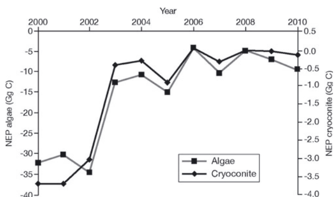
Fig. 7. Carbon flux contributions from algae and cryoconite between 2000 and 2010 predicted using model 4.
