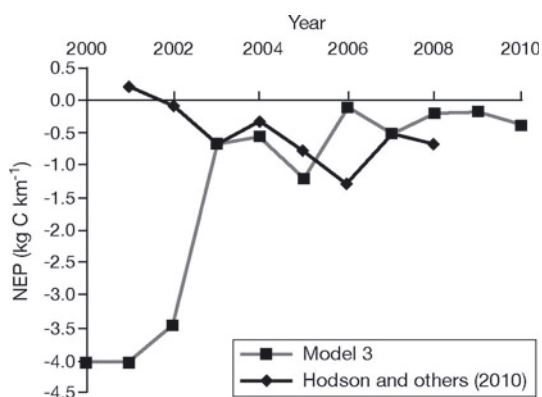
Fig. 5. NEPs as predicted by model 3 and by Hodson and others (2010).
