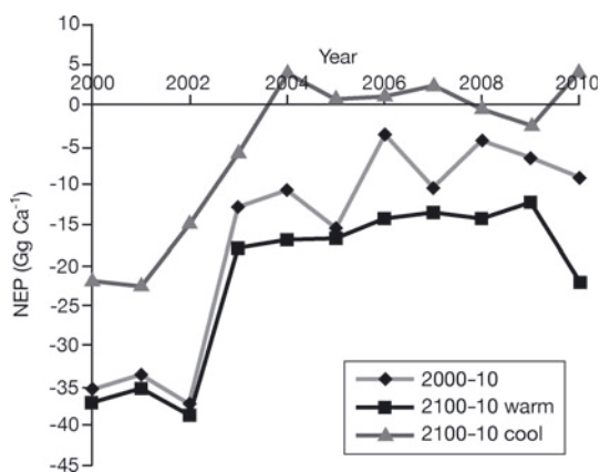
Fig. 9. Net carbon flux as simulated by the present-day, warm GrIS and cool GrIS scenarios.
