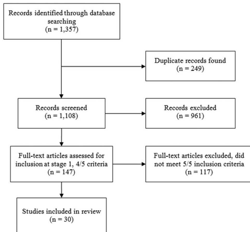
Fig. 1. Search results.
