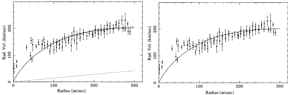
Figure 1. H \alpha Rotation curve with disk + halo (left) and pure disk (right) fits.
