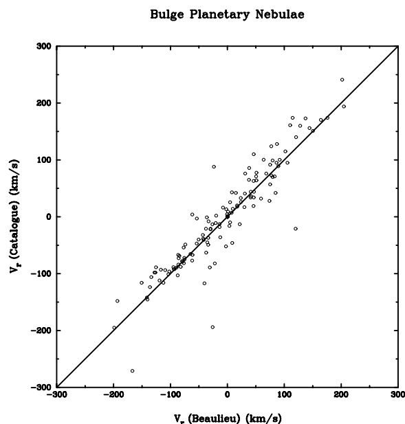
Figure 2 —Comparison between the velocity values obtained from the 74-inch telescope and the catalogued values.
