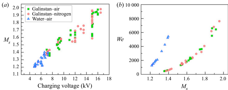
Figure 2. Range of non-dimensional numbers. (a) Variation of shock Mach number ( M_s ) with the capacitor charging voltage of a pulse power system. (b) Variation of Weber number ( We ) with shock Mach number ( M_s ). Similar Weber number values are maintained for comparing Galinstan–air, Galinstan–nitrogen and water–air test cases.
