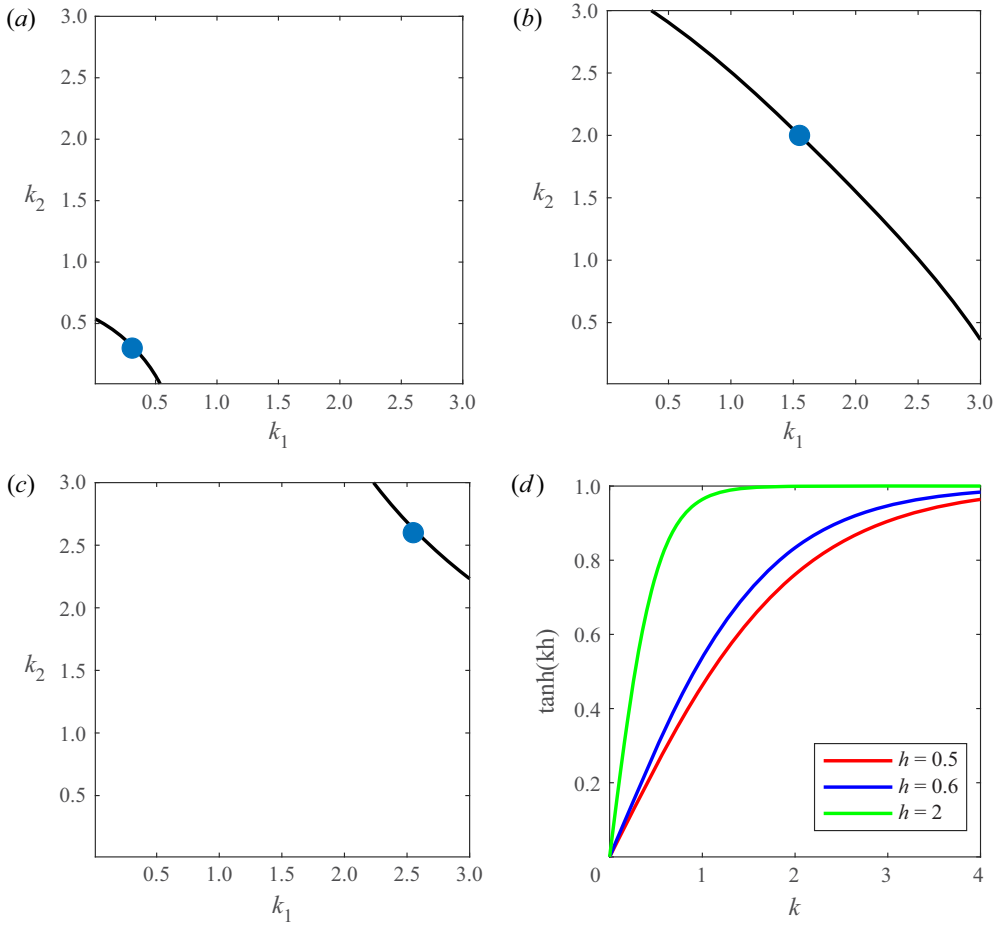
Figure 1. One-dimensional resonant triad curves satisfying the wavenumber–frequency resonance condition k_3 = k_1 + k_2 and \omega_3 = \omega_1 + \omega_2 . All wavenumbers are measured in units of \text{cm}^{-1} and depth h in cm. The numerical values for the depth h and surface tension used to produce the figure are respectively given by (a) h = 0.5 cm; \sigma = 81 \text{ cm}^3 \text{ s}^{-2} , (b) h = 0.6 cm; \sigma = 81 \text{ cm}^3 \text{ s}^{-2} and (c) h = 2 cm; \sigma = 73 \text{ cm}^3 \text{ s}^{-2} . Shown in (d) is the graph of the tanh function for various values of depth. The full circles indicate typical wavenumber values leading to (a) shallow-depth limit with k_1 h \approx 0.15 ; k_2 h \approx 0.15 and k_3 h \approx 0.3 ; (b) finite depth with k_1 h \approx 0.9 ; k_2 h \approx 1.2 and k_3 h \approx 1.5 ; and (d) infinite-depth limit when k_1 h \approx 5 ; k_2 h \approx 5.2 and k_3 h \approx 10.2 .
