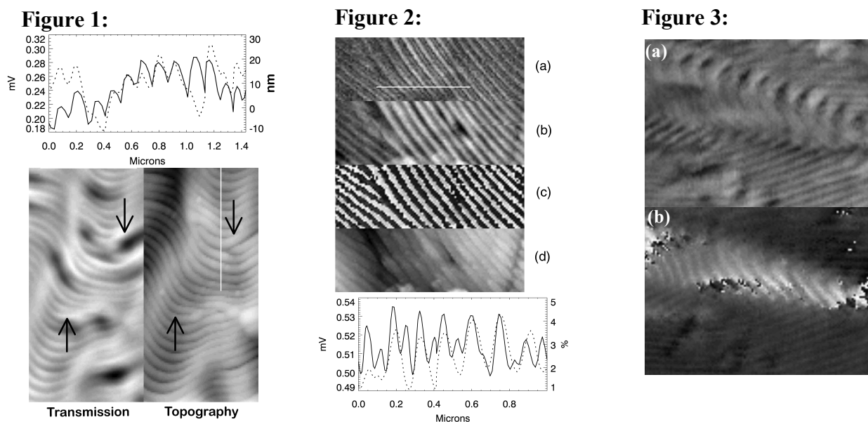
Fig. 1. NSOM micrograph of PS-b-PI. The top plot shows topography (dotted) and transmission (solid) along the white line (1.4 \mu\text{m} ) in the topography image. Arrows indicate edge defects.
