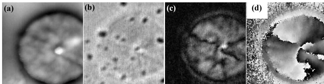
Fig. 4. PM NSOM of PS spherulite. Images are 6x6 \mu\text{m} . (a) topography [43nm], (b) transmission [0.2-0.25mV (a.u.)], (c) Birefringence (retardance) [6°], (d) Birefringence angle (fast axis) [180°].
