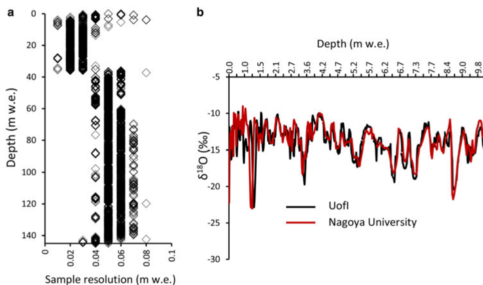
Fig. 3. The profiles of (a) sample length in the BI2003 ice core and (b) oxygen stable isotope ratios, \delta^{18}O (‰). The results received in Uofl and validated with corresponding isotope data at Nagoya University.
