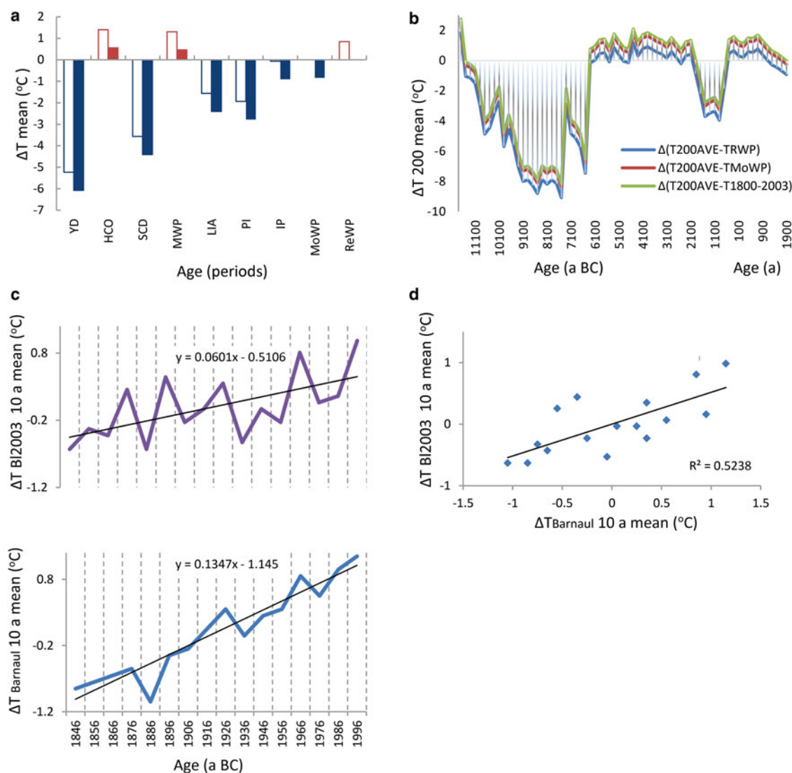
Fig. 8. (a) Average estimations on reconstructed air temperature deviations, \Delta T , ( ^{\circ}\text{C} ) from the Recent (filled column: red is for positive and blue is for negative deviations) and Modern (not filled) Warm Periods for the different historical periods. (b) Bicentennial deviations of reconstructed air temperature from the Recent (green) and Modern (red) Warm Period mean of air temperatures and the last bicentennial mean (blue). (c) Decadal mean deviations from the last decadal mean of air temperature reconstructed from BI2003 ice-core records and from Barnaul Station. (d) Correlation between deviations from the last decadal mean of decadal air temperature means at the Barnaul Station and reconstructed from the BI2003 ice-core records.
